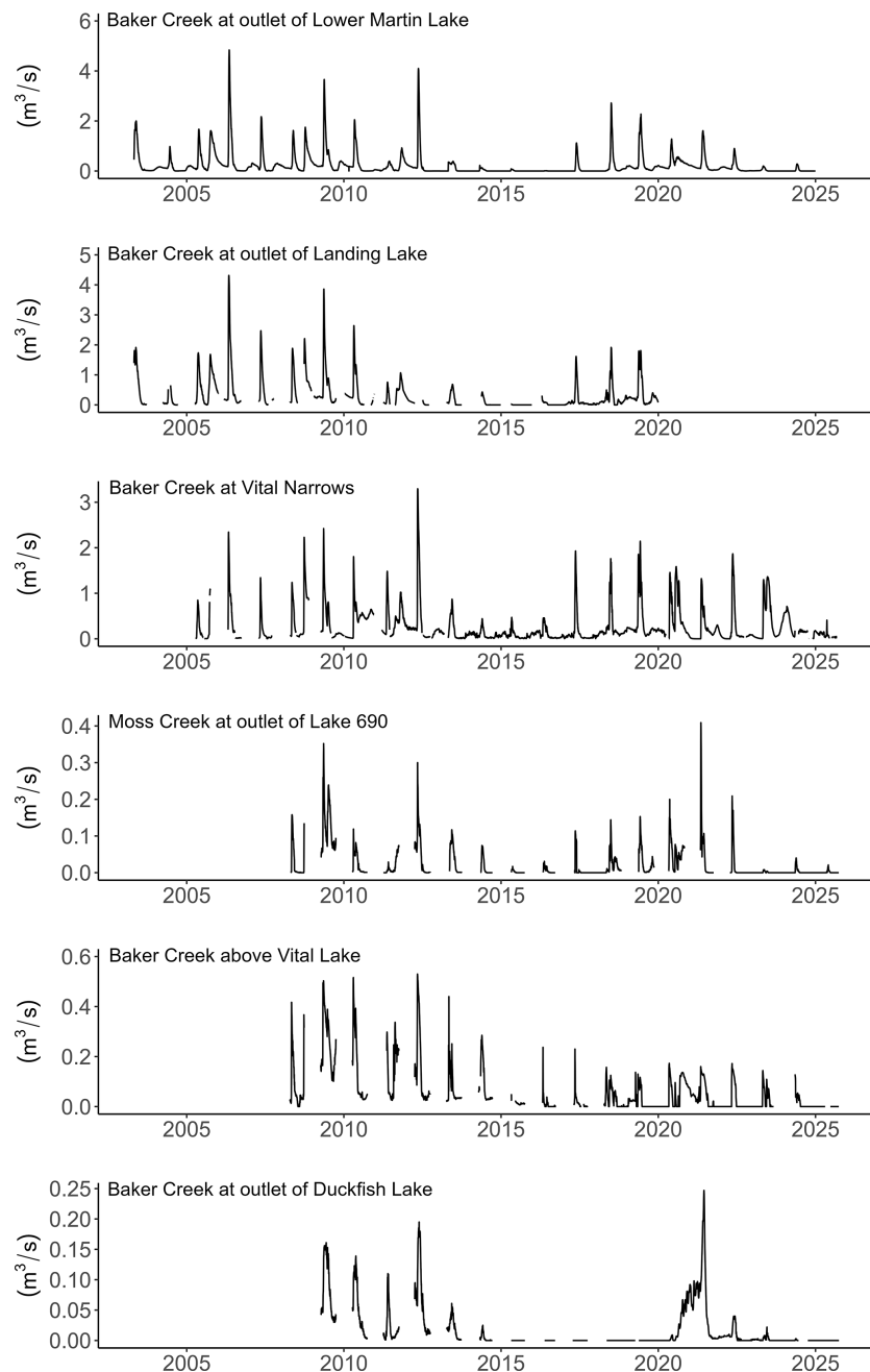
Figure 8. Daily streamflow at the nested hydrometric gauges.
