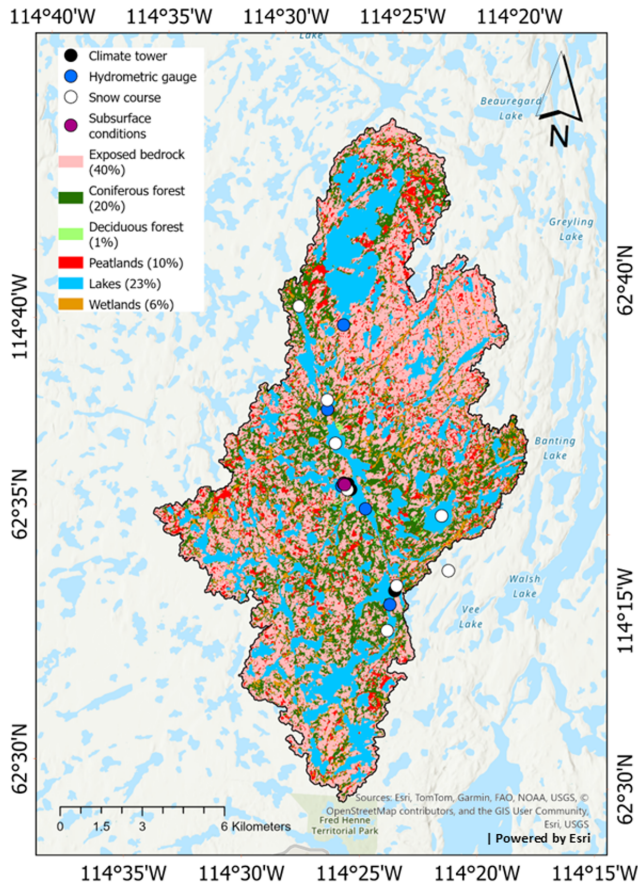
Figure 1. Extent of the Baker Creek Research Watershed illustrating land cover distribution and locations of instrumentation. Background map layer developed by ESRI | Powered by ESRI using sources from ESRI Canada, TomTom, Garmin, SafeGraph, METI/NASA, USGS, EPA, USDA, NRCan, Parks Canada and Esri.
