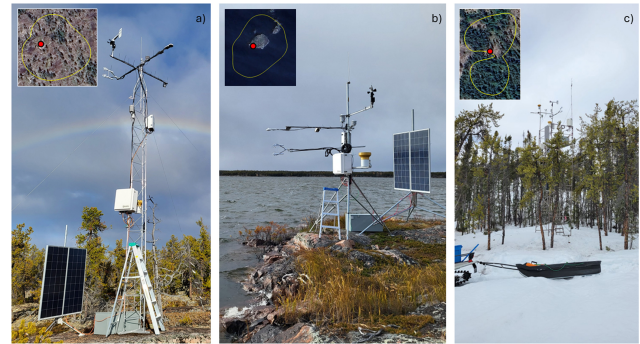
Figure 2. Climate towers (a) on the bedrock ridge; (b) at Landing Lake and (c) the coniferous forested lower hillslope. Inserts illustrate tower footprints within which 90 % of the measurement tends to occur. Authors are the creators/copyright holders of the oblique photos. Satellite imagery: © 2026 Airbus, Map data: © 2026 Google Earth.
