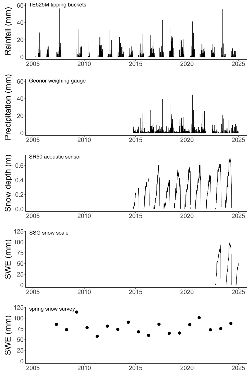
Figure 5. Precipitation time series from April 2005 to December 2024 from (top to bottom); maximum daily rainfall from the tipping buckets, daily precipitation from the Geonor weighing gauge, snow depth measured at the forested hillslope tower, snow water equivalent measured at the snow scale, and watershed average snow water equivalent measured using the annual snow survey. Gaps in rainfall, precipitation, snow depth and snow water equivalent time series because of sensor inoperability or inactivation are evident from breaks in the time series.
