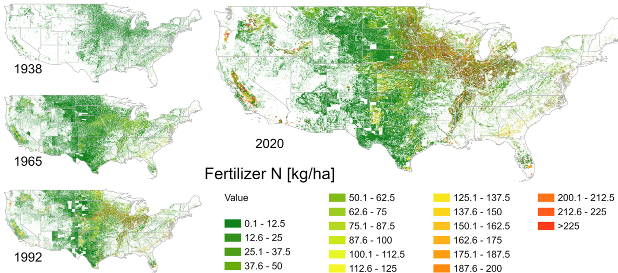
Figure 6. Fertilizer N inputs at 48 arcsec resolution for 1938, 1965, 1992, and 2020 estimated by this study (HLNID).
