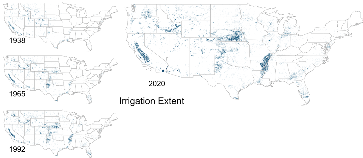
Figure 8. Irrigation extent at 48 arcsec resolution for 1938, 1965, 1992, and 2020 estimated by this study (HLNID).
