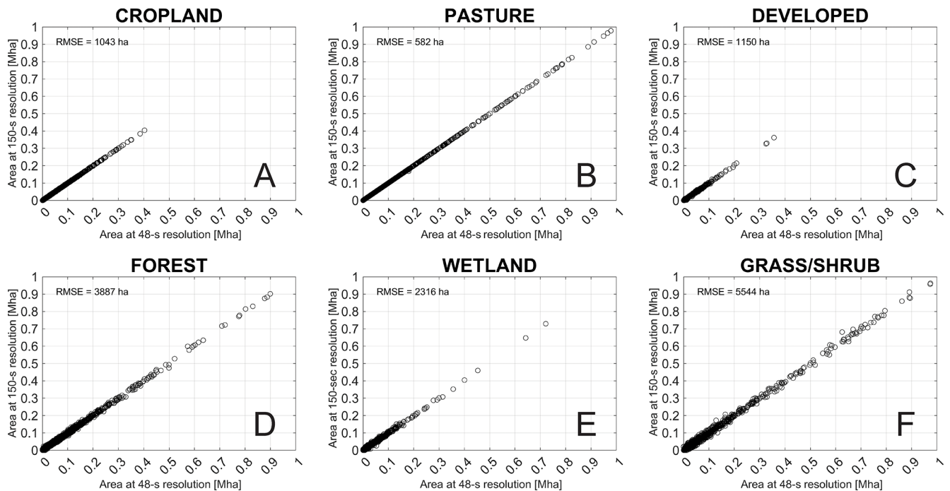
Figure 10. Comparison of estimated areas for 6 LULC types for the year 2020 in each CONUS county at 48 and 150 arcsec resolution with error reported as root-mean-squared-error (RMSE).
