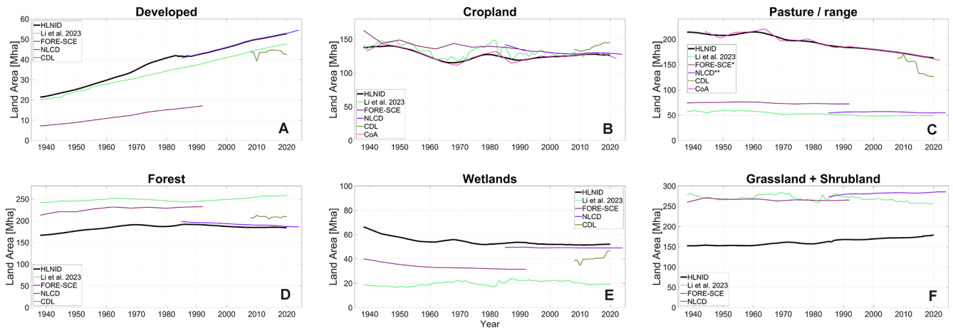
Figure 4. Comparison of land use-land cover areas from 1938–2020 estimated by this study and other datasets: Li et al. (2023), FORE-SCE, NLCD, CDL, and CoA (see Table 1).
