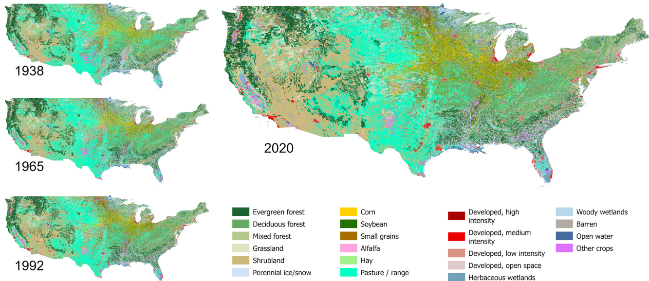
Figure 2. Land use-land cover at 48 arcsec resolution for 1938, 1965, 1992, and 2020 estimated by this study (HLNID).
