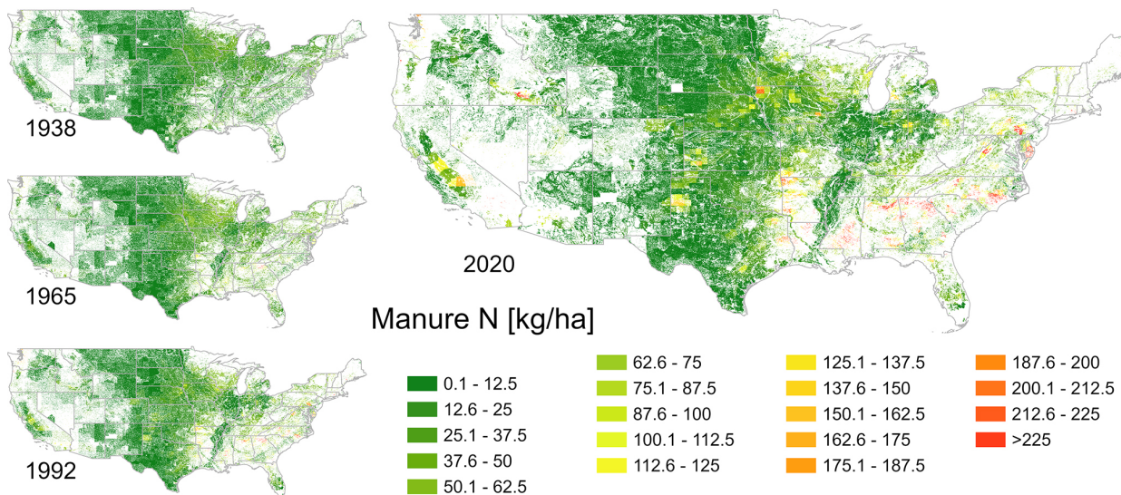
Figure 7. Manure N inputs at 48 arcsec resolution for 1938, 1965, 1992, and 2020 estimated by this study (HLNID).
