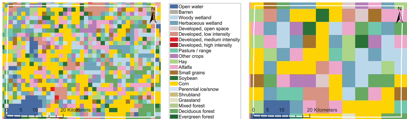
Figure 9. Land use-land cover maps at 48 (left) and 150 (right) arcsec resolution of a representative county (Jefferson, WI) in 1980.
