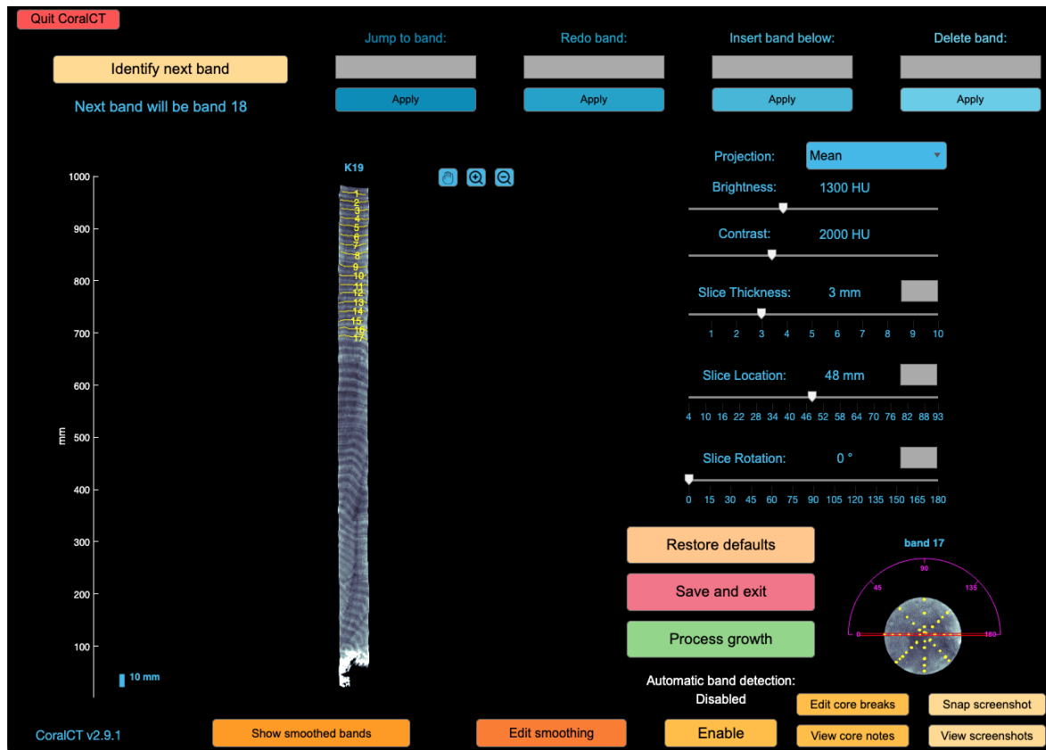
Figure 1. Default display of a partially-analyzed coral skeletal core in the CoralCT application. Sliders found on the right side of the screen are used to adjust the cores appearance to increase visual clarity of annual density bands. In the core image, clear alternations of high-density (bright) and low-density (dark) bands are visible, with a pair of high- and low-density bands together representing one year of growth. The yellow lines and digits indicate user-defined bands. On this core, the observer has identified bands as the darkest part of low-density bands. In the axial image toward the lower-right, the current slice location is displayed by the red box, and yellow dots indicate the distribution of tie-points for the present band (band 17 in this case). Additional descriptions of the methods of the CoralCT application can be found in DeCarlo et al. (2025b).
