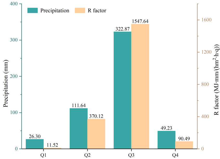
Figure 16. Quarterly rainfall in 2024 and the corresponding quarterly averaged R factor for the Loess Plateau.
