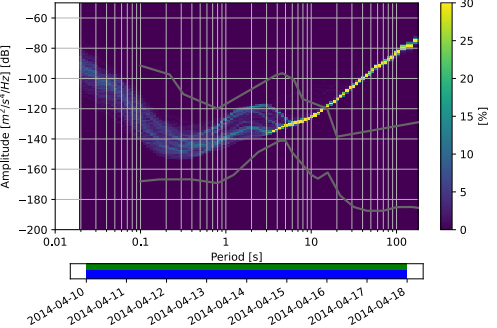
RM.OT06..EHZ 2014-04-10 -- 2014-04-17 (383/383 segments)
