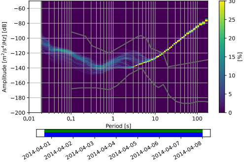
RM.OT08..EHE 2014-03-31 -- 2014-04-07 (351/351 segments)
