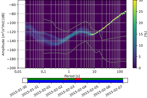
RM.OT07..EHN 2015-01-30 -- 2015-02-06 (383/383 segments)
