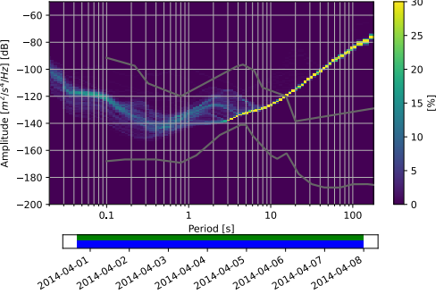
RM.OT08..EHZ 2014-03-31 -- 2014-04-07 (351/351 segments)
