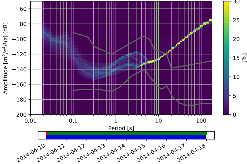
RM.OT06..EHN 2014-04-10 -- 2014-04-17 (382/382 segments)
