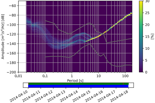
RM.OT06..EHE 2014-04-10 -- 2014-04-17 (382/382 segments)
