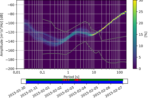
RM.OT07..EHZ 2015-01-30 -- 2015-02-06 (383/383 segments)
