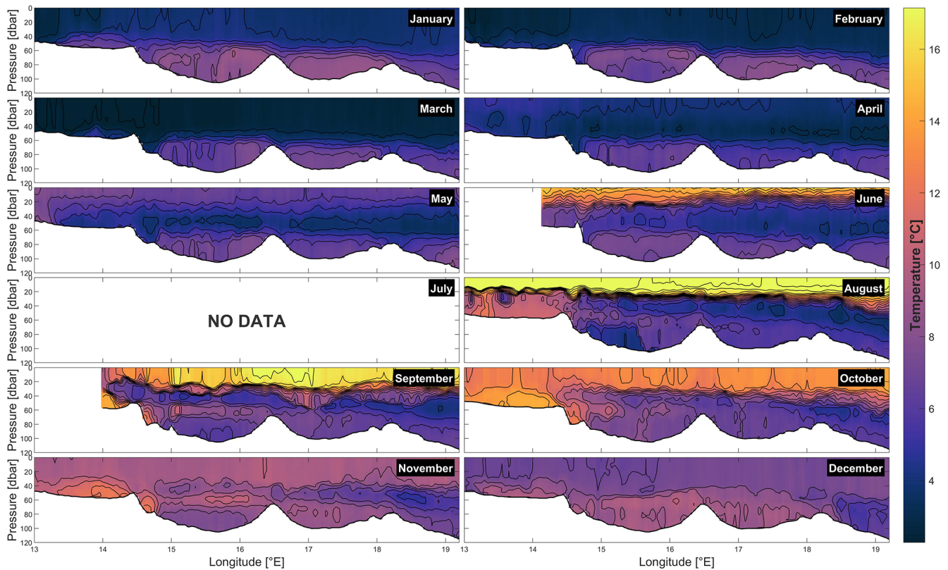
Figure 8. Monthly mean temperature sections (January–December) along the Baltic transect as a function of longitude ( ^{\circ} E) and pressure (dbar).
