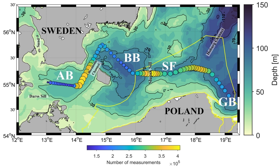
Figure 1. Spatial distribution of CTD profiles collected during R/V Oceania cruises between 1997 and 2024 in the southern Baltic Sea. The yellow line indicates the Polish Exclusive Economic Zone (EEZ). The labels AB, BB, SF and GB denote the Arkona Basin, Bornholm Basin, Stupsk Furrow and Gdańsk Basin, respectively.
