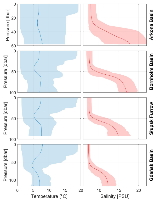
Figure 7. Basin-mean vertical profiles of temperature and salinity in the Arkona Basin, Bornholm Basin, Słupsk Furrow and Gdańsk Basin derived from all CTD casts collected along the repeat section between 1997 and 2024. Solid lines indicate the multi-year mean and shaded envelopes the full range (min–max) across all cruises.
