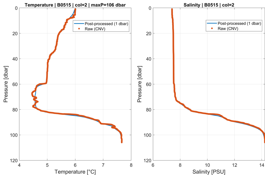
Figure 6. Example of a raw CTD profile and the same profile after post-processing. Raw CNV samples (dots) and the 1 dbar product (solid line) are shown for temperature ( ^{\circ}\text{C} ) and salinity (PSU); pressure increases downward (dbar).
