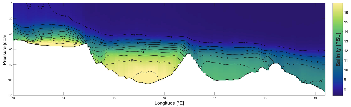
Figure 9. Mean salinity (1997–2024) section along the repeat Baltic transect, shown as a function of longitude ( ^{\circ} E) and pressure (dbar).
