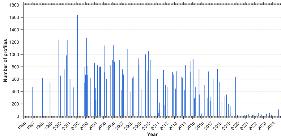
Figure 4. Distribution of CTD profiles conducted by IOPAN along the main monitoring transect in the southern Baltic Sea.
