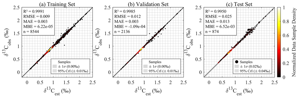
Figure A3. GPR model evaluation for numerical model \delta^{13}\text{C}_{\text{DIC}} reconstruction (observation-constrained sparse sampling): Density scatter plots comparing GPR model-estimated ( \delta^{13}\text{C}_{\text{est}} ) versus numerical model outputs \delta^{13}\text{C}_{\text{DIC}} ( \delta^{13}\text{C}_{\text{obs}} ) values during (a) training, (b) validation, and (c) independent testing.
