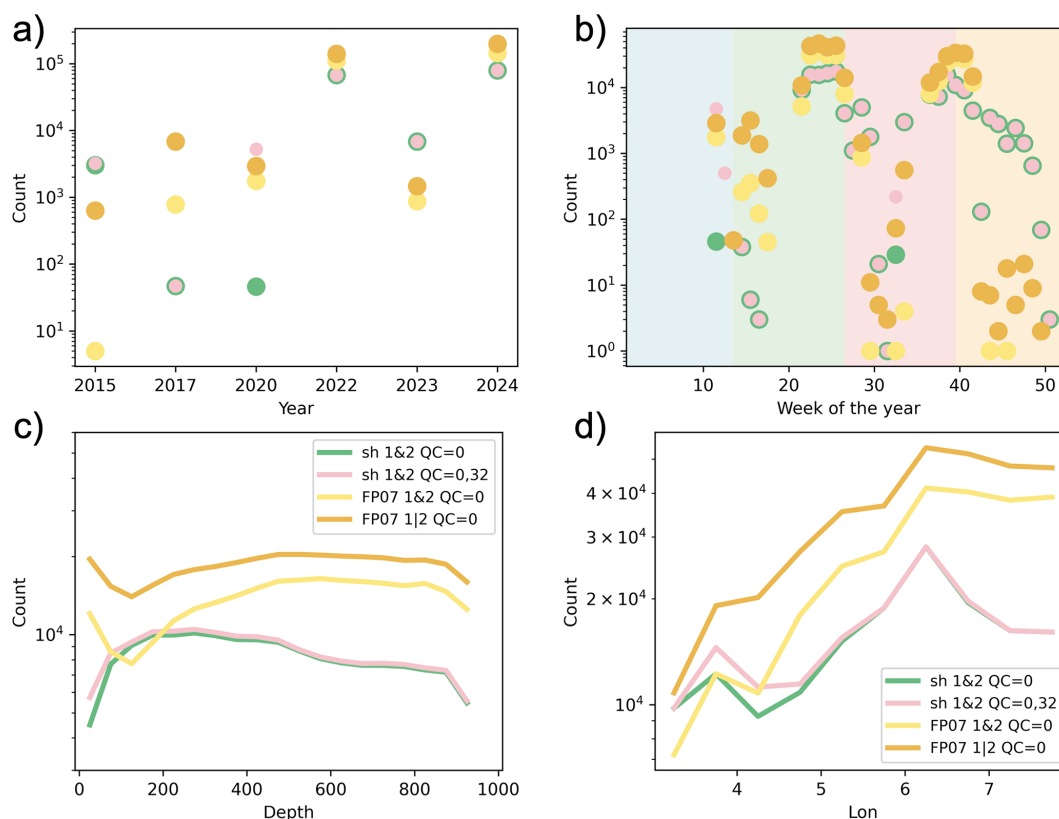
Figure 7. Count of passing data by bins of: years, week of the year, depth, and longitude. Green indicates the (best) cross-probe choice for shears and pink as a secondary cross-probe choice considering a relaxed despiking fraction criteria. Yellow indicates that both FP07 estimates pass; orange one on two.
