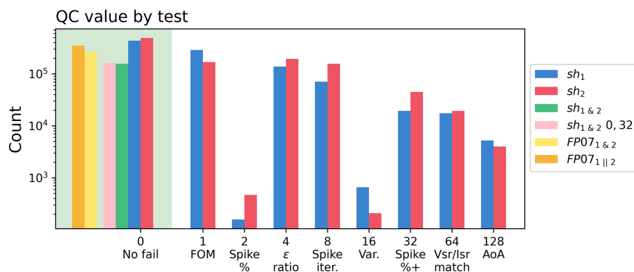
Figure 6. Count of the primary QC flags. Blue and red respectively refer to sh_1 , sh_2 probes. Green indicates the (best) cross-probe choice and pink as a secondary cross-probe choice considering a relaxed despiking fraction criteria. Yellow indicates that both FP07 estimates pass, orange indicates that one of the two passes. Cumulative/combination of flags is not shown.
