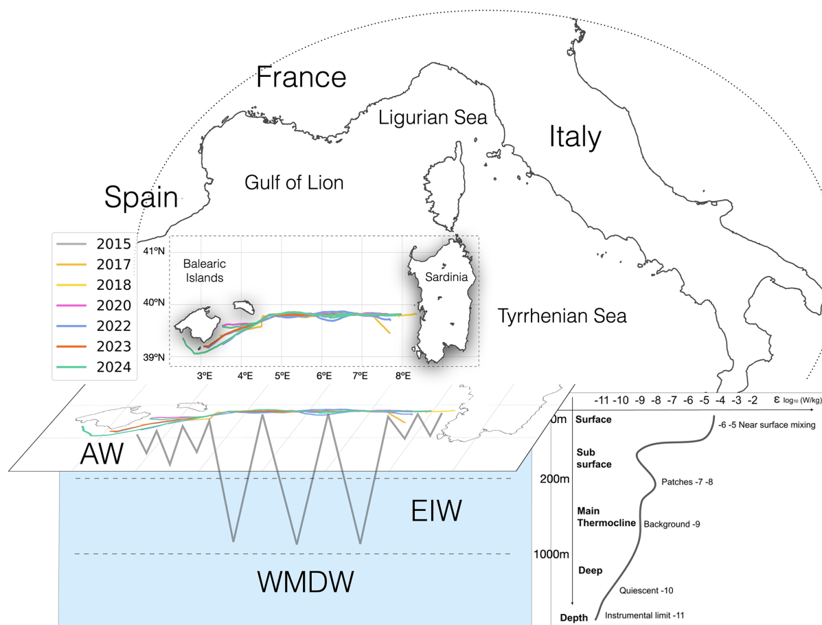
Figure 1. Glider Teresa mission along its longitudinal transect, by years (in colors). The scheme indicates the deployment between Sardinia and Balearic Islands in the Western Mediterranean Sea. Sawtooth black lines indicate a schematic trajectory from surface up to 1000 m-depth, encountering layers of the Atlantic Water (AW) in surface, the Eastern Intermediate Water (EIW) and the Western Mediterranean Deep Water (WMDW). Depth levels associated to these water masses (respectively 0–200 m, 200–1000 m, 1000 m+) are indicative. The lower-right panel provides a schematic representation of typical ranges of turbulent kinetic energy dissipation rates ( \epsilon , logarithmic scale) as a function of depth.
