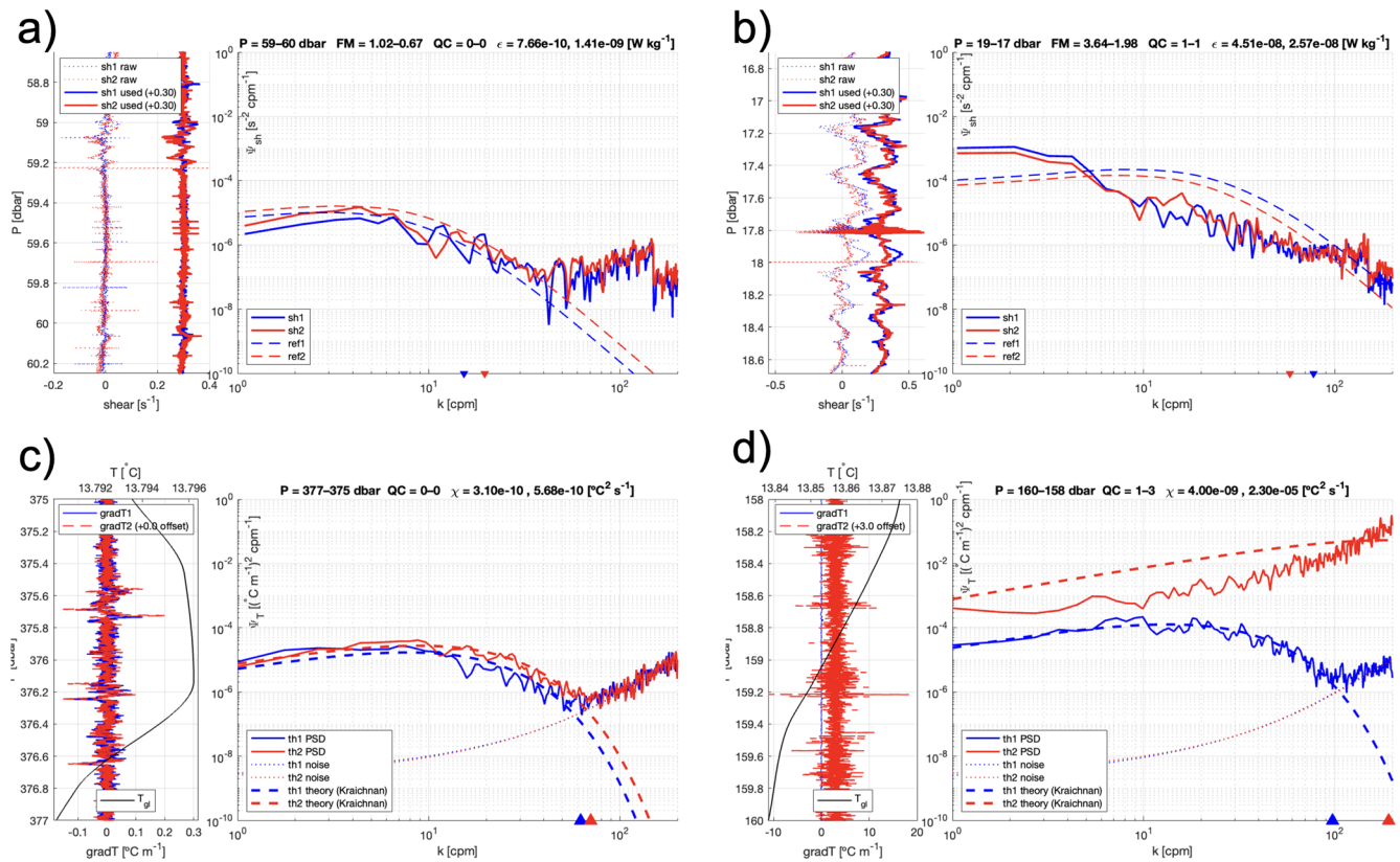
Figure 4. Examples of shear- and thermistor-based spectra illustrating accepted and rejected estimates. Panels (a, b) show shear cases and panels (c, d) thermistor cases. Left subpanels display the raw and retained signals (sh1 in blue, sh2 in red; th1 in blue, th2 in red; glider temperature in black for thermistors) over the dissipation segment. Right subpanels show the corresponding wavenumber spectra. For shear, observed spectra are compared to the Nasmyth model; for thermistors, to the Kraichnan model. Dashed curves indicate the fitted reference spectra; symbols mark the spectral integration limits used to compute \varepsilon or \chi . Panel (a) (23 May 2024) illustrates a fully validated shear case ( QC=0-0 ). Panel (b) (22 May 2024) shows a shear case rejected due to poor spectral fit ( QC=1-1 ; elevated FOM). Panel (c) (12 September 2022) presents a validated thermistor case ( QC=0-0 ). Panel (d) (15 March 2020) shows a thermistor case where one probe fails QC while the other remains acceptable ( QC=1-3 ).
