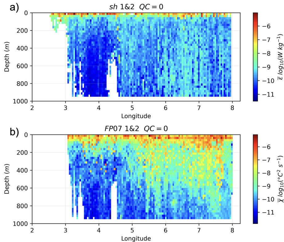
Figure 8. Synthetic sections of all good estimates of \varepsilon and \chi (all years considered) averaged by depth bins of 25 m, and longitudinal bins of 0.045^\circ (circa 5 km).
