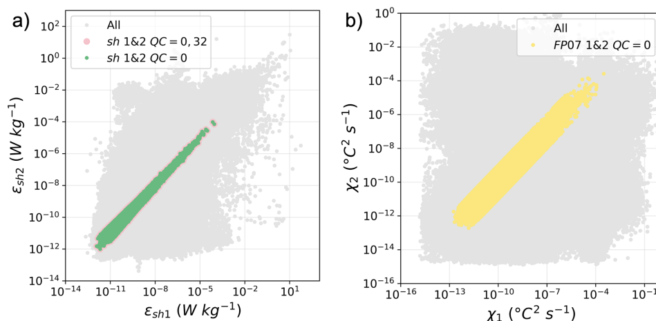
Figure 5. Scatter plots of cross-checked estimates of (\varepsilon_1, \varepsilon_2) and (\chi_1, \chi_2) . Gray points indicate all estimates; (a) green indicates the (best) cross-probe choice; (b) yellow indicates that both FP07 estimates pass.
