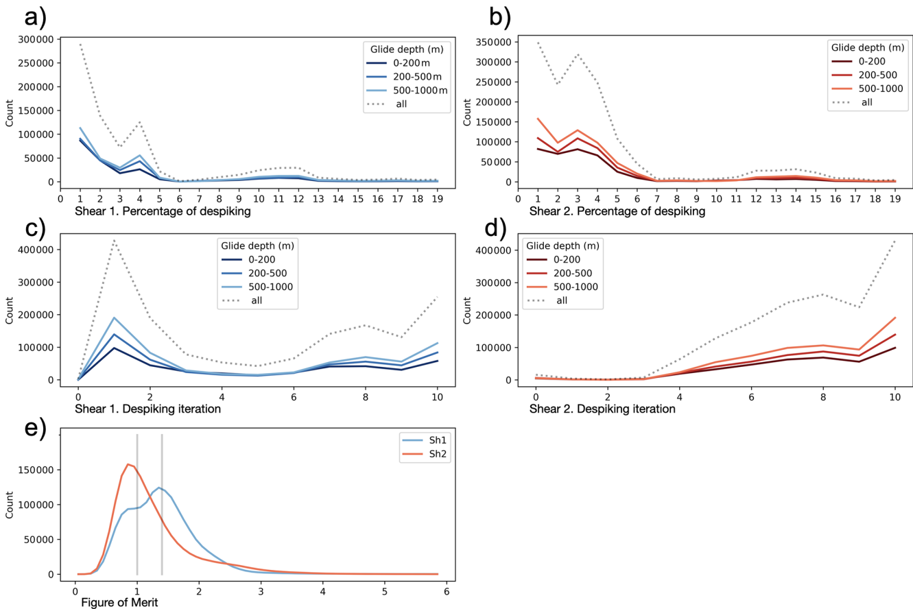
Figure 3. Count of spiking fraction (a, b) and pass count (c, d) for shear 1 (blue) and shear 2 probes (red), by bins of glider depth extension, in meter (i.e. from short to long glide). Count of FOM values (e) for shear 1 (blue) and shear 2 (red).
