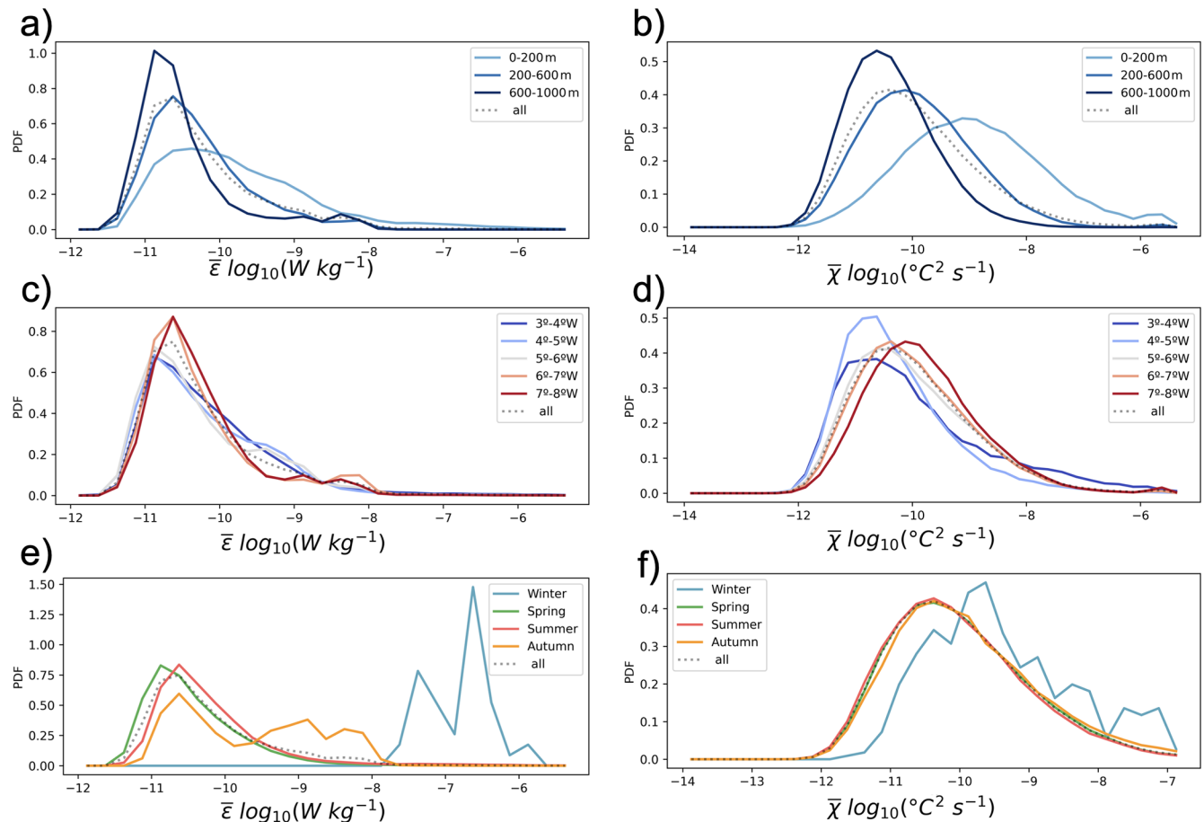
Figure 9. Normalized probability distribution functions (PDF) of cross-checked passing ( QC=0 ) estimates of \varepsilon (a, c, e) and \chi (b, d, f) binned by layers, longitudinal fractions and seasons.
