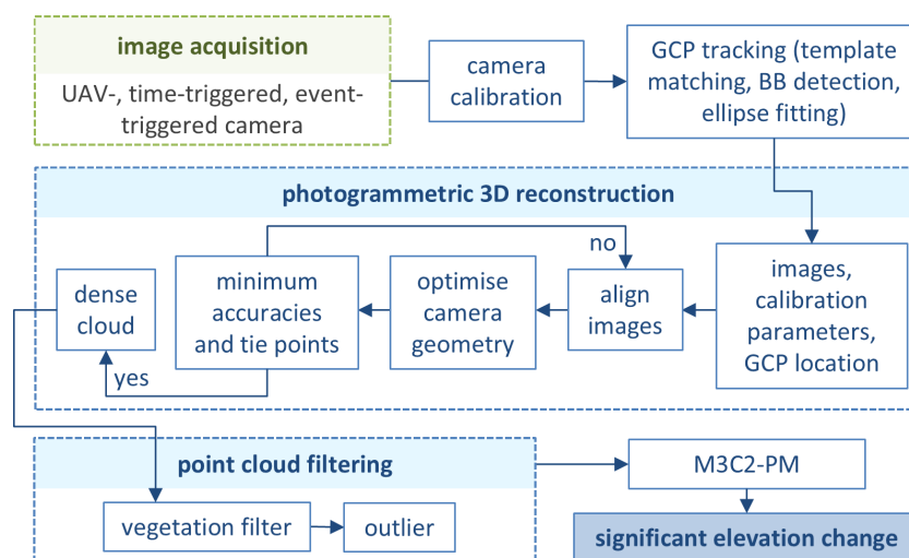
Figure 6. Image processing workflow adapted after Eppe et al. (2025) (GCP = ground control point, M3C2 PM = Multiscale Model to Model Cloud Comparison with Precision Maps, BB detection = bounding box detection).
