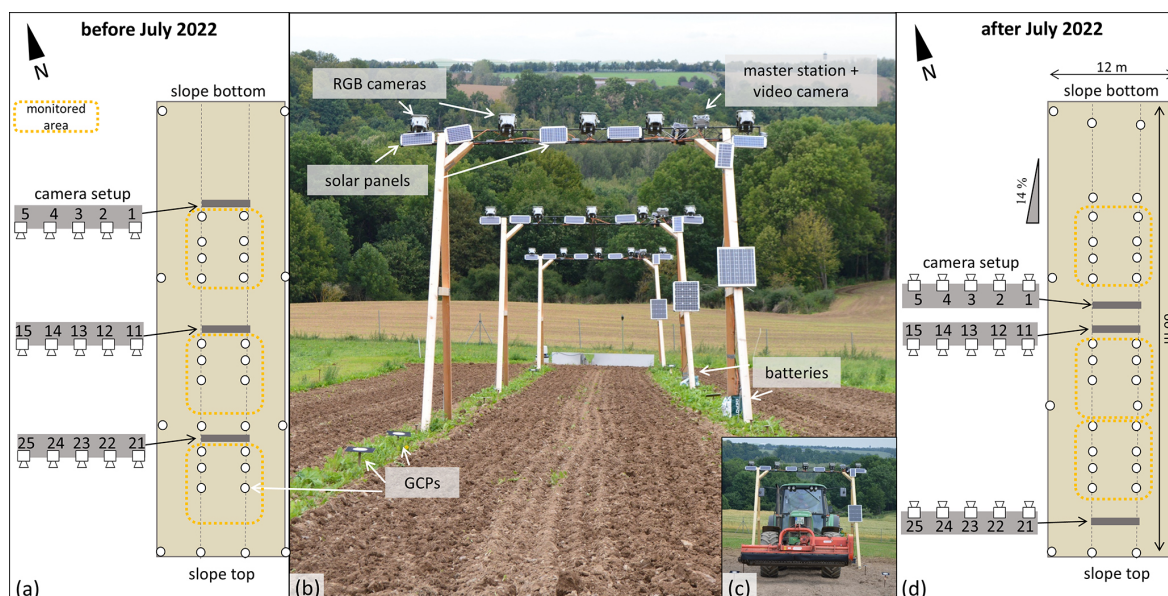
Figure 4. Monitoring setup on the slope scale with three monitoring stations, each equipped with five RGB cameras (b). The schematic representation in (a) and (d) includes the camera designations and positions of the GCPs (ground control points). Panel (a) presents the setup employed until July 2022. Subsequently a slight modification was implemented as shown in (d). The height of the posts was chosen to facilitate the mechanical removal of vegetation (c) while minimising potential restrictions.
