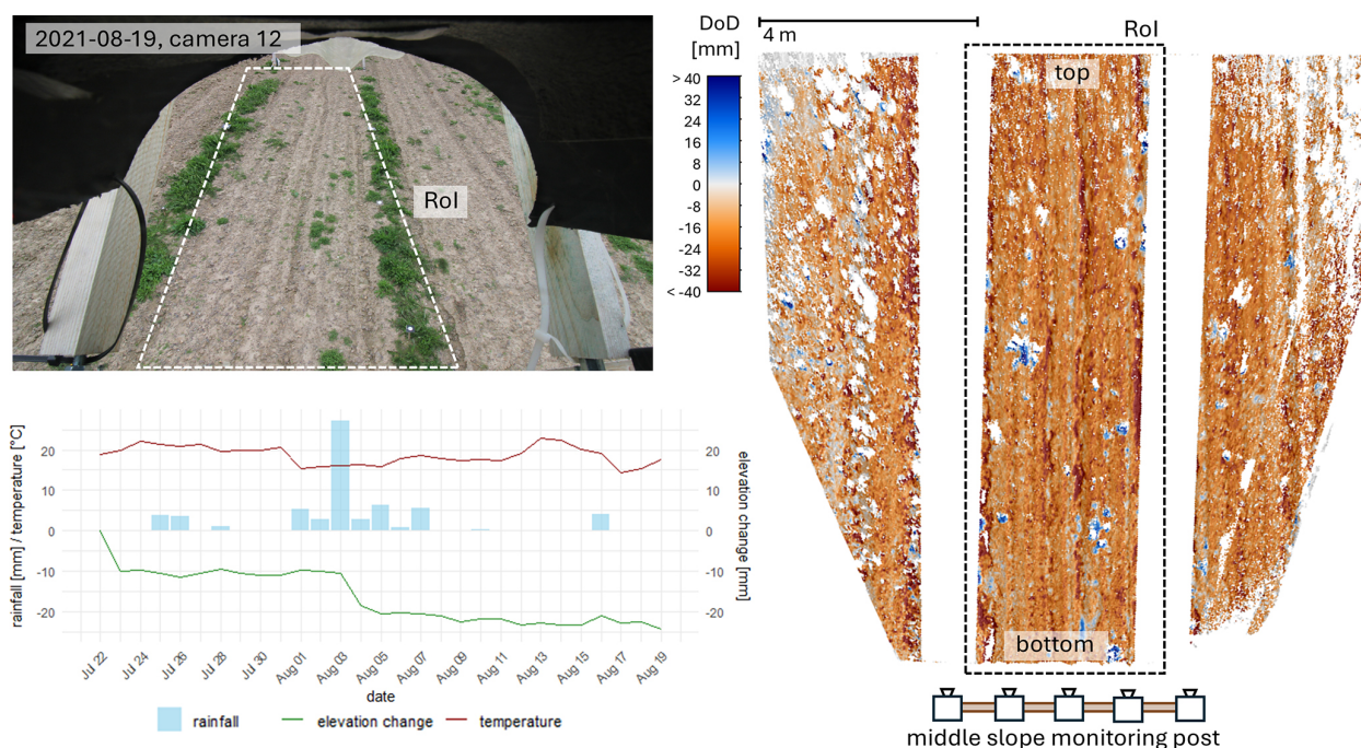
Figure 8. Results of a 28 d observation time at the middle slope position in July and August 2021. At the top: image of the camera 12, taken on 19 August 2021 at 10:00 a.m. At the bottom: timeline for the period 22 July 2021 (right after tillage) until 19 August 2021 (day before tillage), with the average M3C2 elevation change, the temperature and the daily rainfall. To the right: DoD (digital elevation model of difference) subtracting the days 22 July and 19 August 2021, with the schematic illustration of the middle slope monitoring post (bottom), cameras facing upslope. The RoI (region of interest) is marked by the dotted black/white box.
