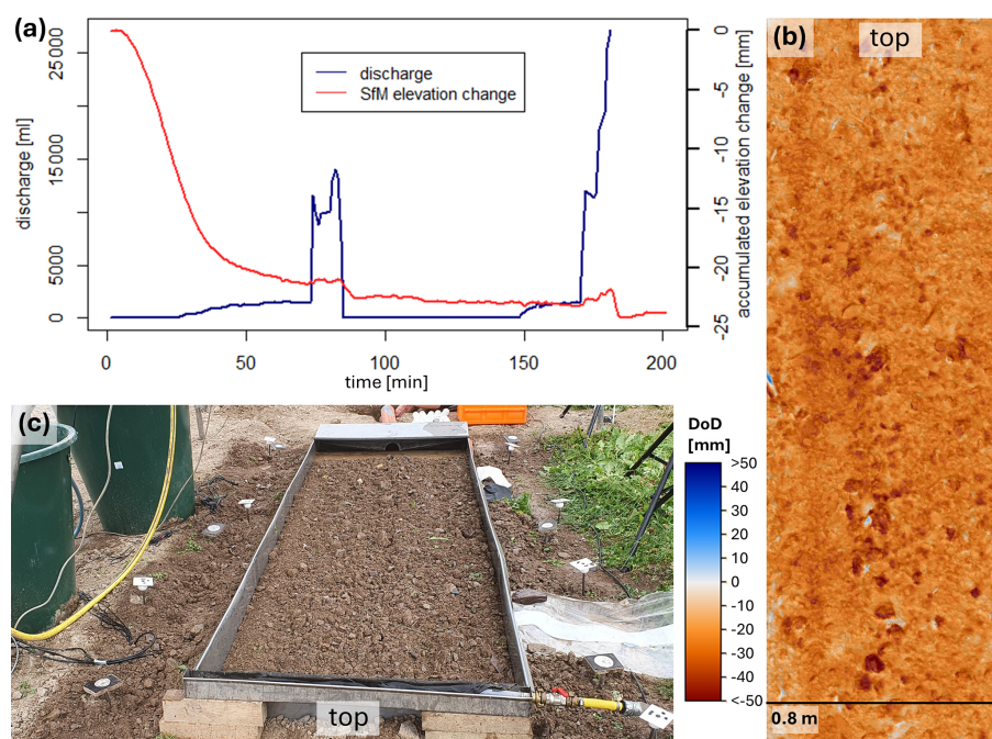
Figure 7. Rainfall simulation results on 21 July 2021 on the plot scale. (a) Timeline of the accumulated spatial averaged elevation change measured via SfM (structure from motion) and the measured discharge at the plot's outlet covering the whole simulation time. (b) DoD (digital elevation model of difference) subtracting the dense clouds captured before and after the rainfall simulation presenting the spatially distributed elevation change. (c) Image of the rainfall simulation plot, shortly after the start.
