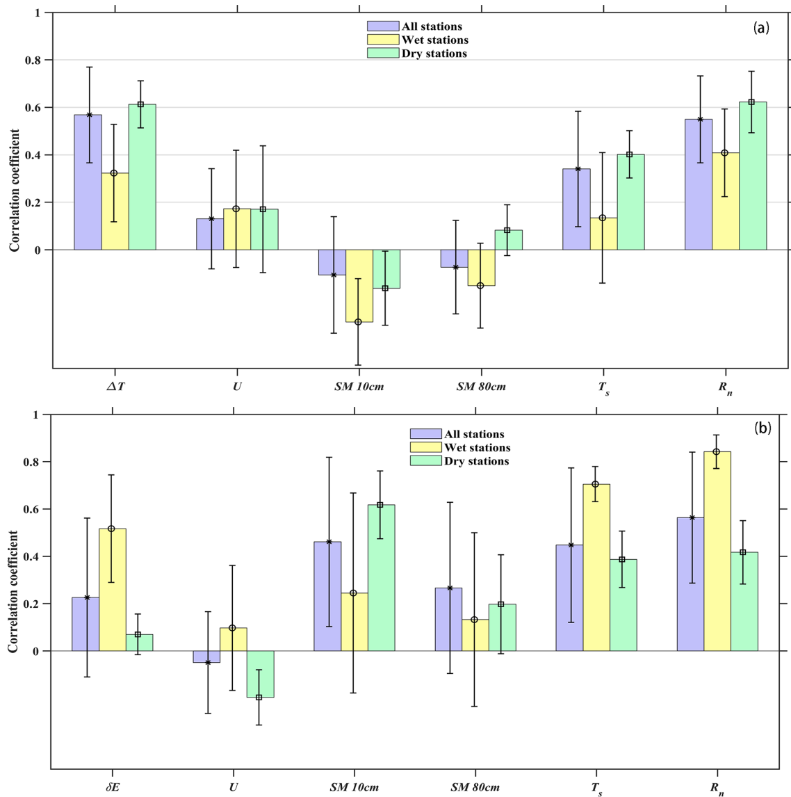
Figure 5. The correlation coefficients between sensible heat flux (a), latent heat flux (b) and related environmental variables at a temporal resolution of hourly under conditions of all stations, wet stations and dry stations, respectively. The statistical significance of the correlation coefficients for each station is provided in Table S7.
