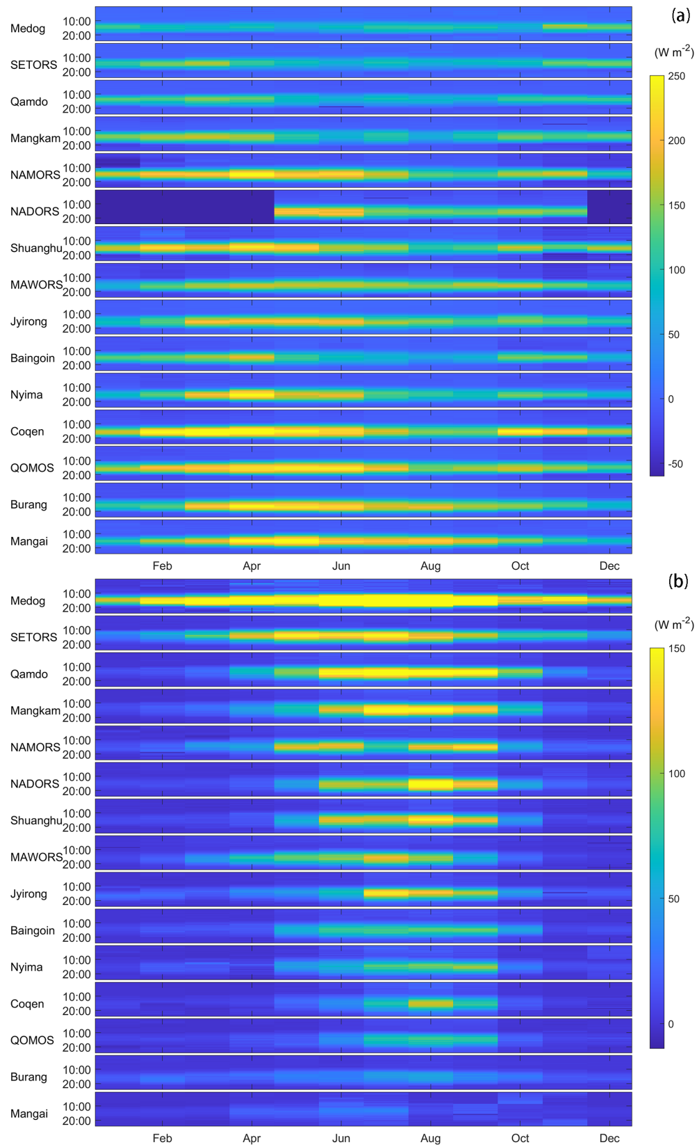
Figure 4. The heat maps for averaged diurnal and seasonal variations of sensible heat flux (a) and latent heat flux (b) at 15 stations.
