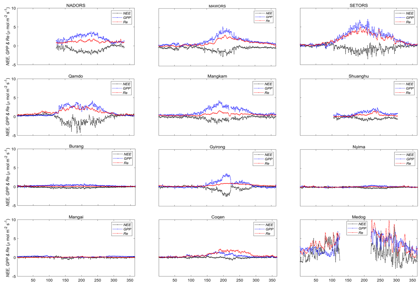
Figure 6. The seasonal variations in NEE, GPP, Re across different sites. The negative NEE values indicated a net uptake of CO 2 . The black, blue and red lines stand for daily NEE, GPP and Re, respectively.
