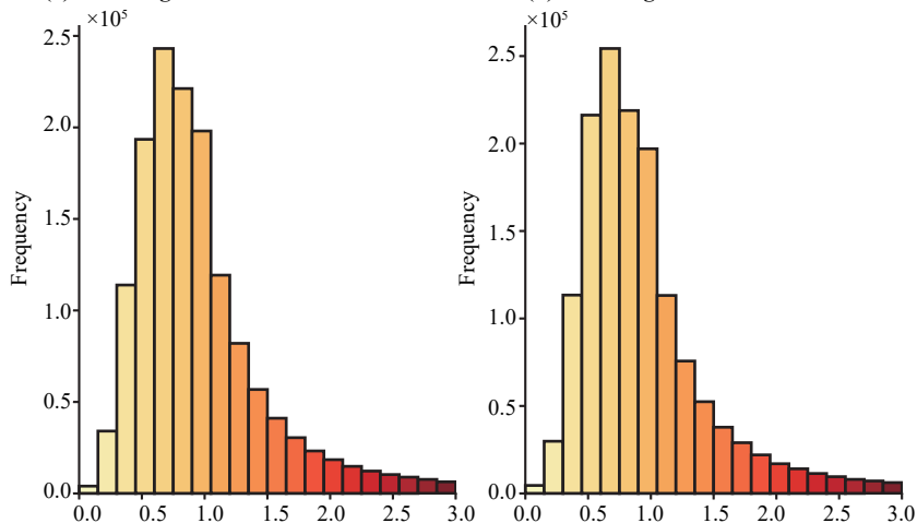
(d) n Histogram for the Wettest 3-Year Period (e) n Histogram for the Driest 3-Year Period (f) ECDF Comparison of Parameter n Distributions
