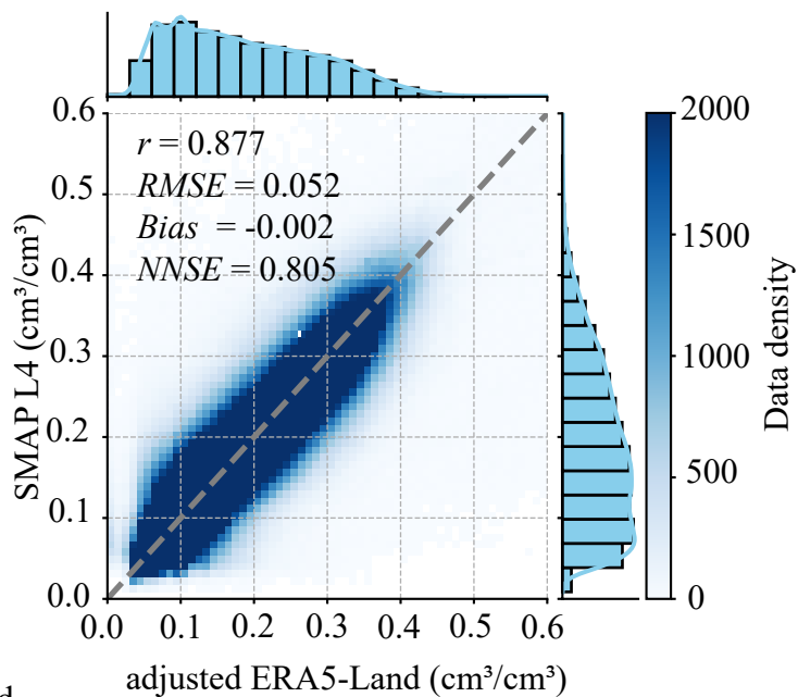
(f) Density scatter plot (after adjustment)
