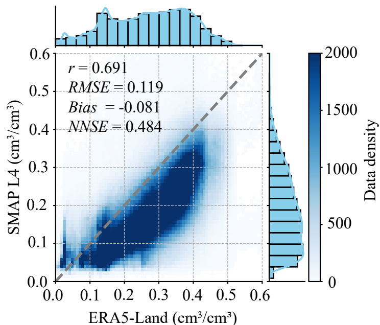
(f) Density scatter plot (after adjustment)
