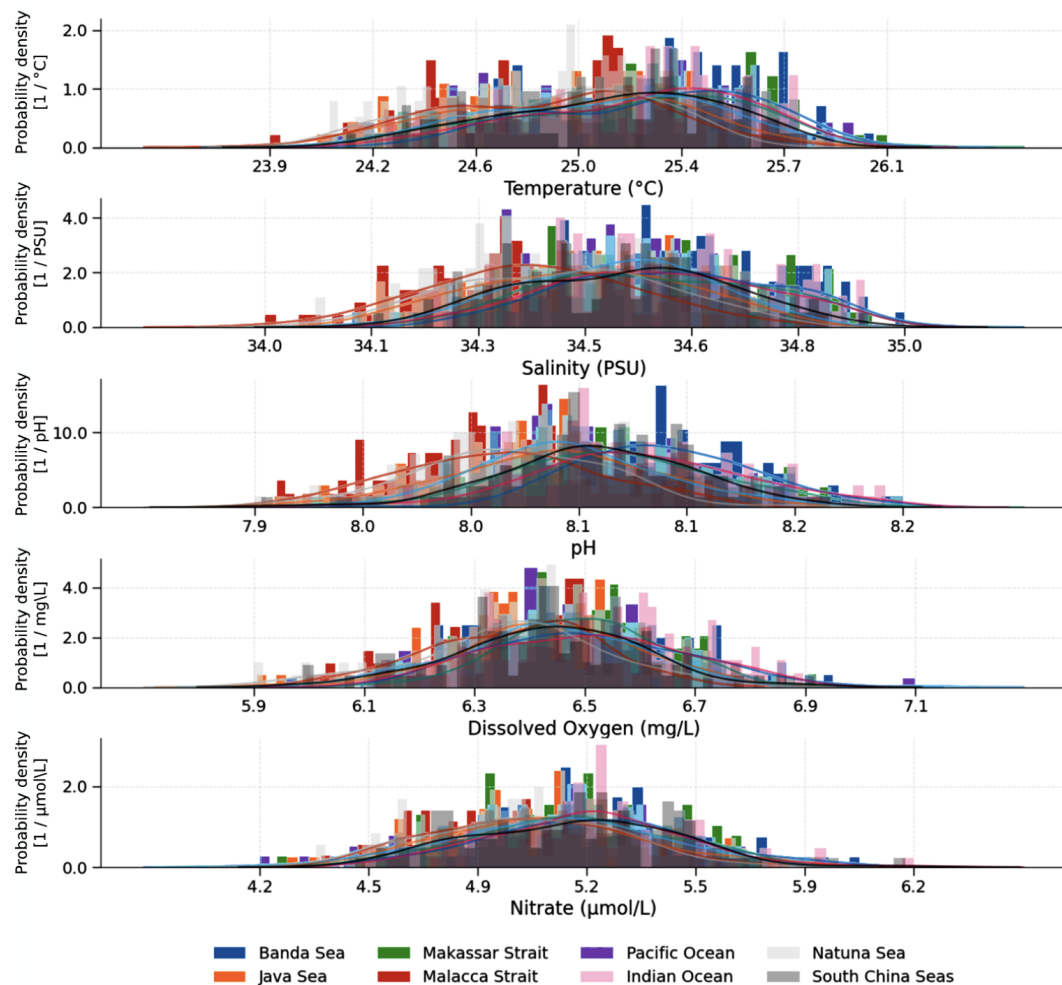
Figure 6. Distribution of five essential ocean variables by region. The histograms (filled colours) show the observed data distribution, while line colours represent the smoothed distribution using the KDE estimation method.
