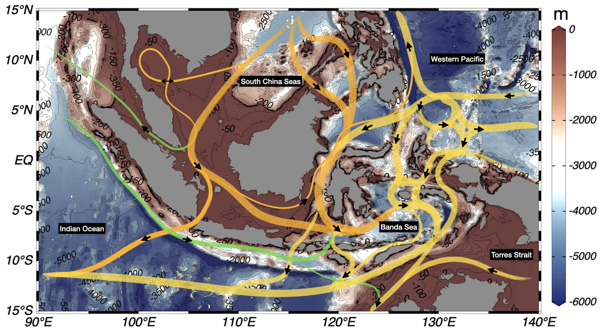
Figure 1. A map of Indonesian seas and surroundings (bathymetric derived from https://www.gebco.net/ , last access: 2 June 2025). Schematic general circulation is presented with lines and adopted from previous findings (Burnett et al., 2000; Gordon, 2005; Shinoda et al., 2012; Susanto et al., 2010). Yellow lines represent water mass from the Pacific Ocean, orange lines represent water mass from the South China Sea (SCS) through the Karimata Strait, and green lines represent water mass from the Indian Ocean.
