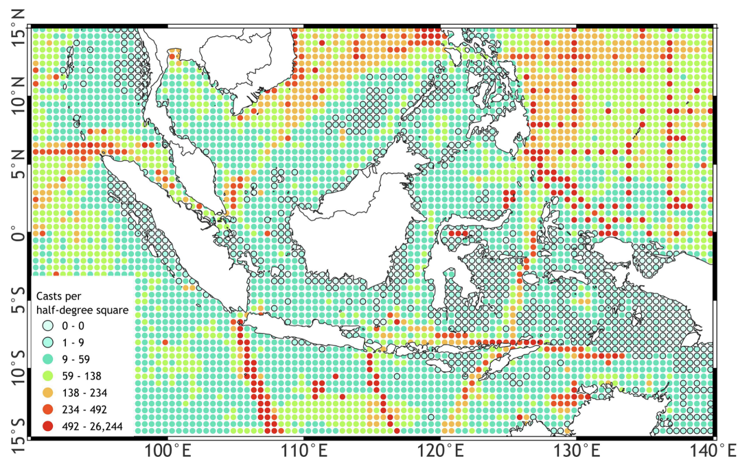
Figure 8. Spatial distribution of historical oceanographic casts per half-degree grid square in the ISS region over the observational period. Cast density is categorized into seven quantiles: Q_0 (no data), Q_1 (1–9 casts), Q_2 (10–59 casts), Q_3 (60–138 casts), Q_4 (139–234 casts), Q_5 (235–492 casts), and Q_6 (493–26 244 casts).
