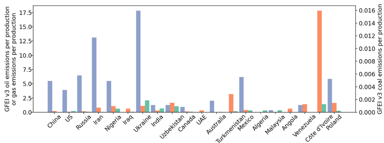
Figure S1: Methane emissions by sector for the top 20 emitting countries (as shown in Figure 2) relative to oil, gas, and coal production. Emissions are from GFEI v3 ( \text{Gg a}^{-1} ) and production data are from EIA (2023) in units of billion cubic feet per year (gas), thousand barrels per day (oil), and thousand short tons per year (coal).
