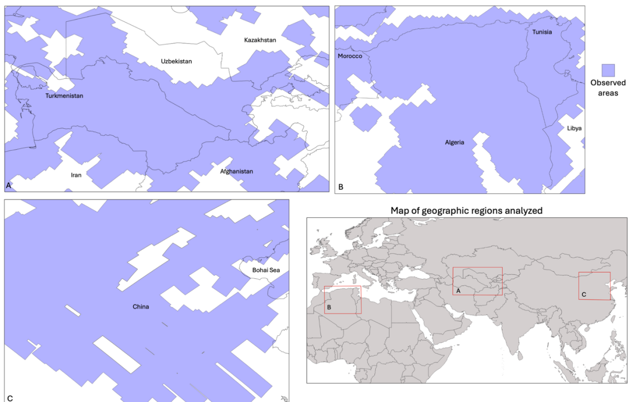
Figure S3: Map of the geographic regions where Carbon Mapper has processed data to look for super-emitting events in Turkmenistan/Uzbekistan (A; top left), Algeria (B; top right), and northeast China (C; bottom left). The bottom right plot shows a zoomed-out map view of the three regions.
