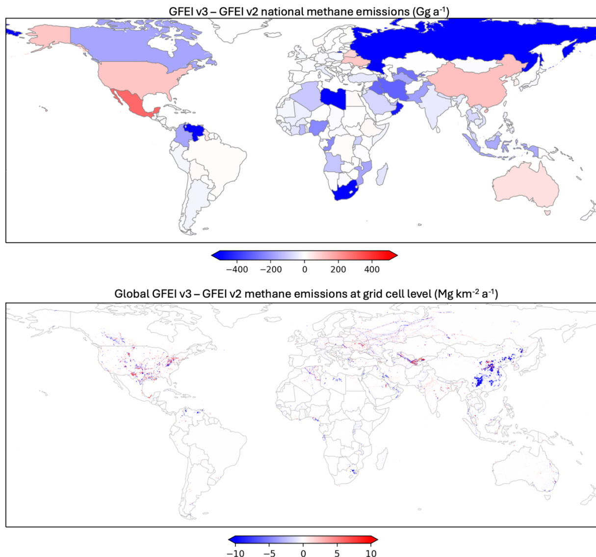
Figure S2: The difference between GFEI v3 and GFEI v2 oil, gas, and coal emissions. The emissions difference between GFEI v3 and v2 is shown at the national scale (top) and per grid cell at native resolution ( 0.1^\circ \times 0.1^\circ ; bottom). In the US, the spatial differences in emissions between the two GFEI versions are primarily a result of the GEPA update from v1 to v2, including oil-gas increases in the Permian (south-central US) and coal decreases in Appalachia (northeast US).
