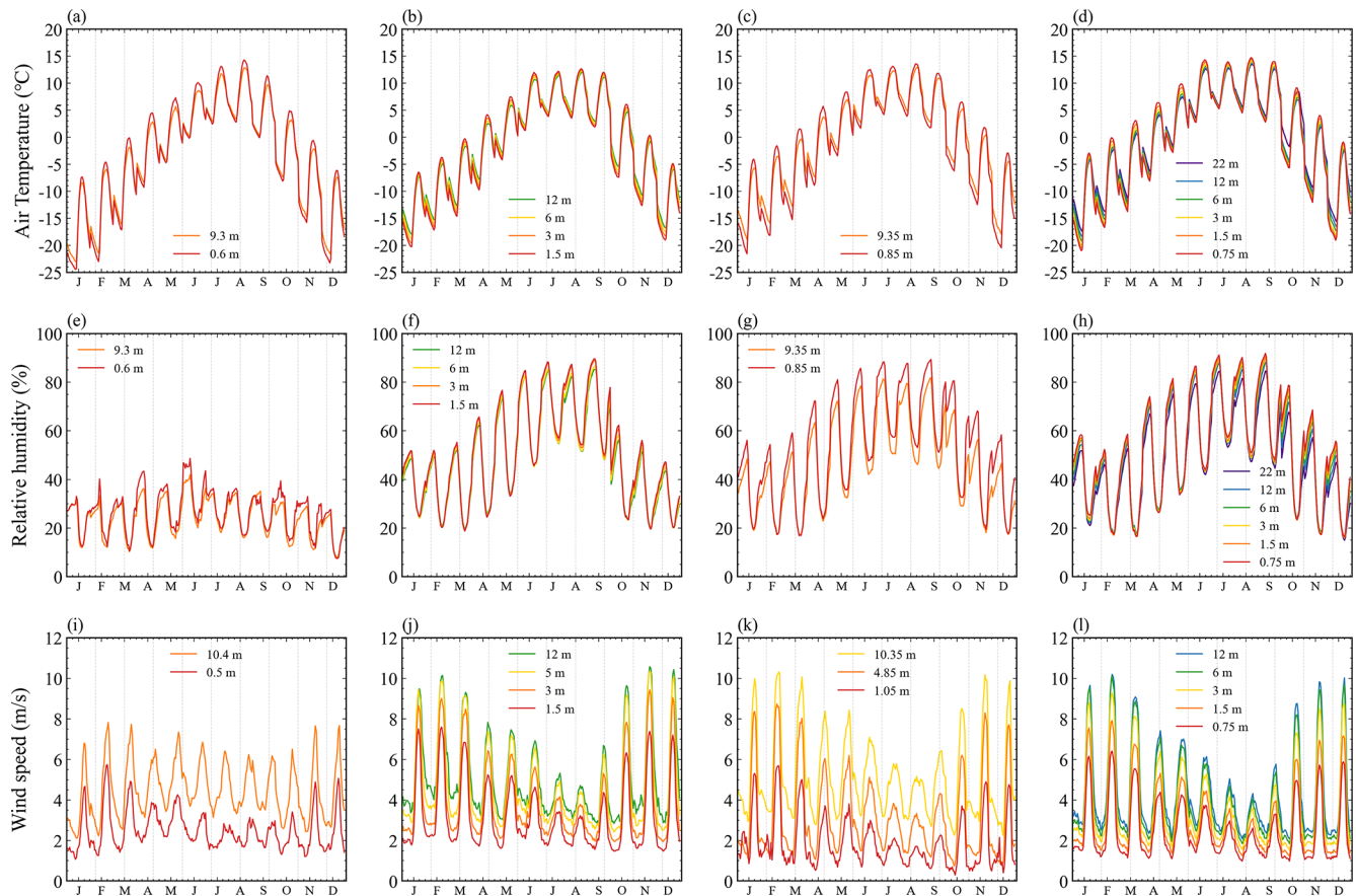
Figure 3. Monthly diurnal variations of temperature at different heights of the PBL tower at NewD66 (a), Amdo (b), MS3478 (c) and BJ (d), with corresponding relative humidity (e–h) and wind speed (i–l) at each station.
