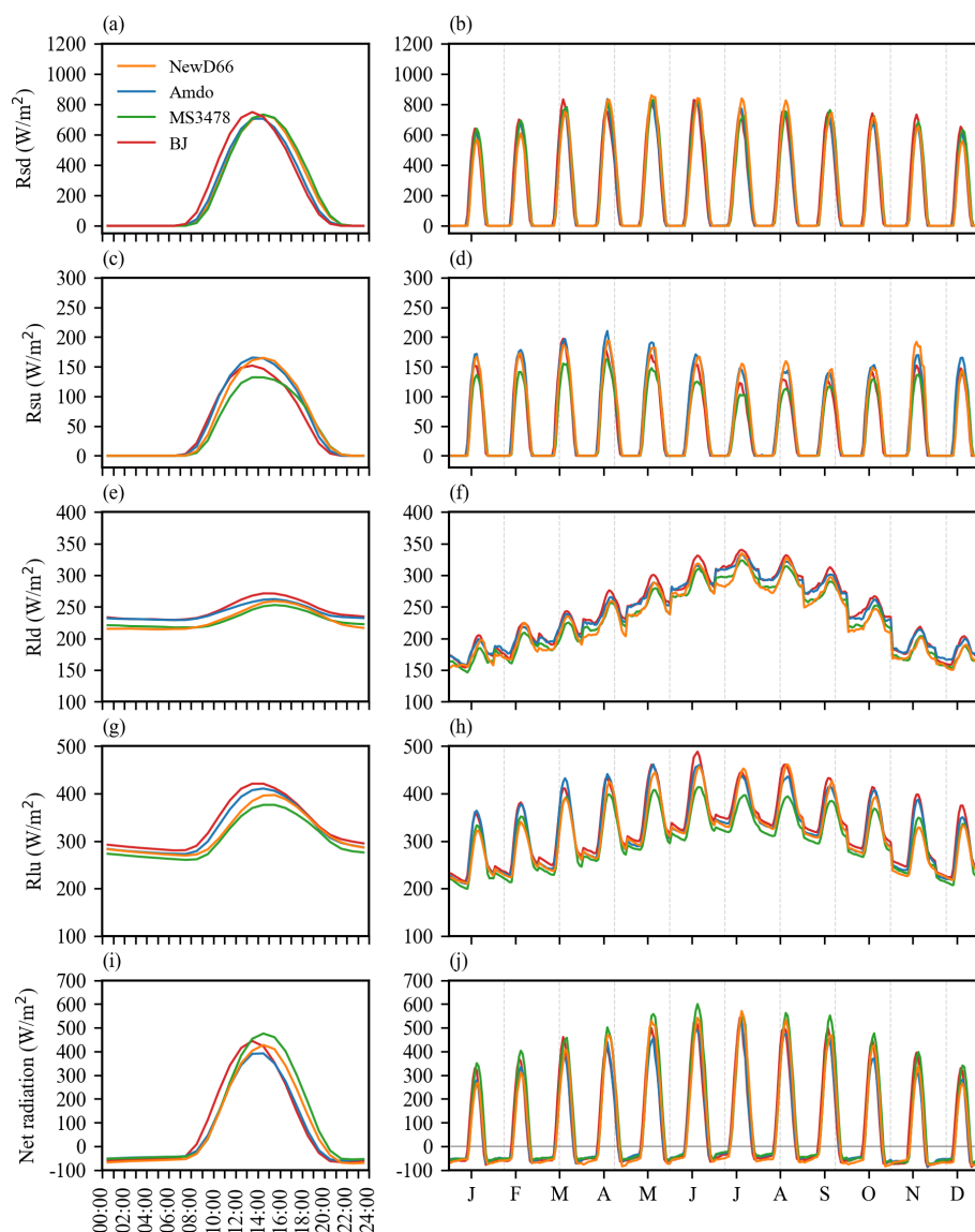
Figure 6. Diurnal variations (a, c, e, g, i) and monthly variations of the diurnal (b, d, f, h, j) downward shortwave radiation (a, b), upward shortwave radiation (c, d), downward longwave radiation (e, f), upward longwave radiation (g, h), and net radiation (i, j) at the 4 stations.
