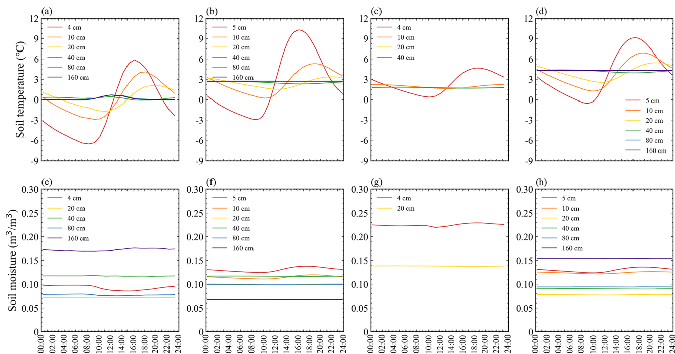
Figure 9. Layered soil temperature at NewD66 (a), Amdo (b), MS3478 (c), and BJ (d) observation, and corresponding layered soil moisture (e–h) at each station.
