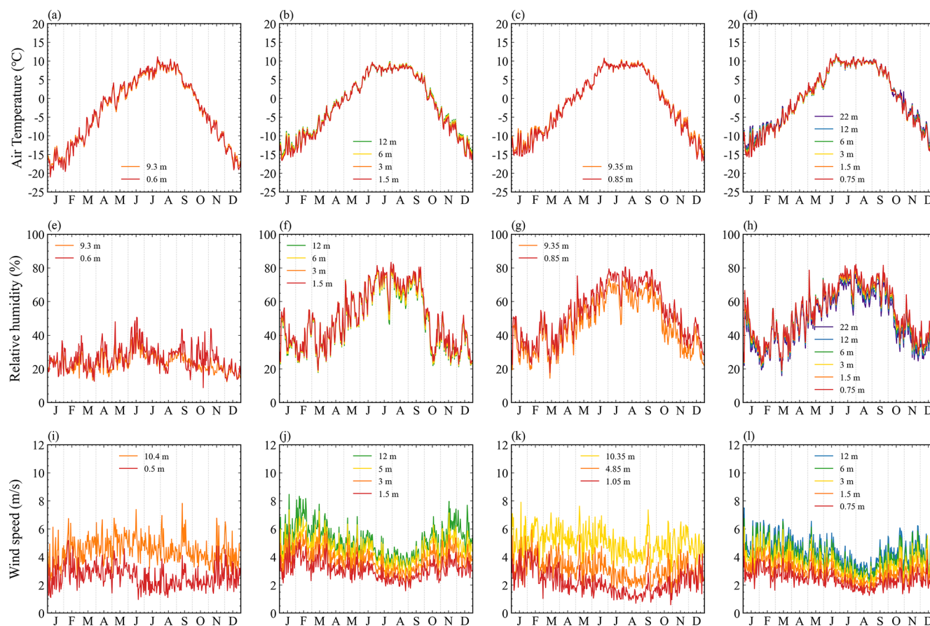
Figure 4. Daily mean of temperature at different heights of the PBL tower at NewD66 (a), Amdo (b), MS3478 (c) and BJ (d), with corresponding relative humidity (e–h) and wind speed (i–l) at each station.
