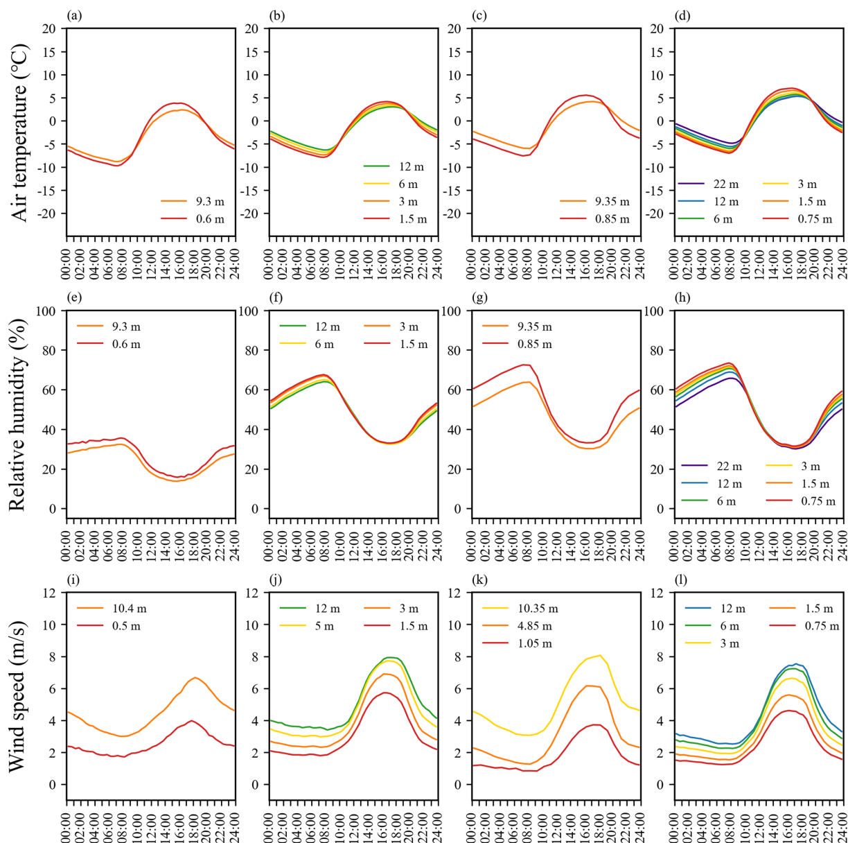
Figure 2. Diurnal variations of temperature at different heights of the PBL tower at NewD66 (a), Amdo (b), MS3478 (c) and BJ (d), with corresponding relative humidity (e–h) and wind speed (i–l) at each station.
