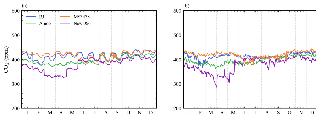
Figure 8. Monthly variations of the diurnal (a) and daily mean (b) \text{CO}_2 concentration at the 4 stations.
