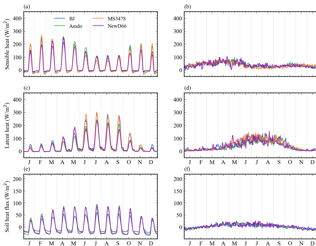
Figure 7. Monthly variations of the diurnal (a, c, e) and daily mean (b, d, f) sensible heat (a, b), latent heat (c, d), and soil heat flux (e, f) at the 4 stations.
