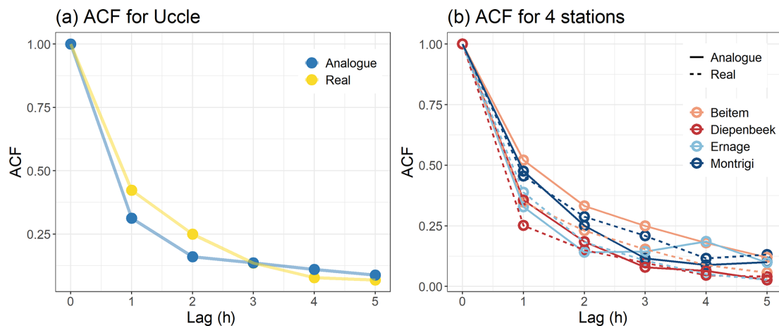
Figure 14. (a) Autocorrelation Function (ACF) for hourly data from Uccle in 2006, comparing real hourly AWS data with median hourly radar data based on the 10 best analogs in Uccle in 2006. (b) ACF for hourly data from Beitem, Mont Rigi, Ernage en Diepenbeek in 2006 on real and best analog days using lag period of 5.
