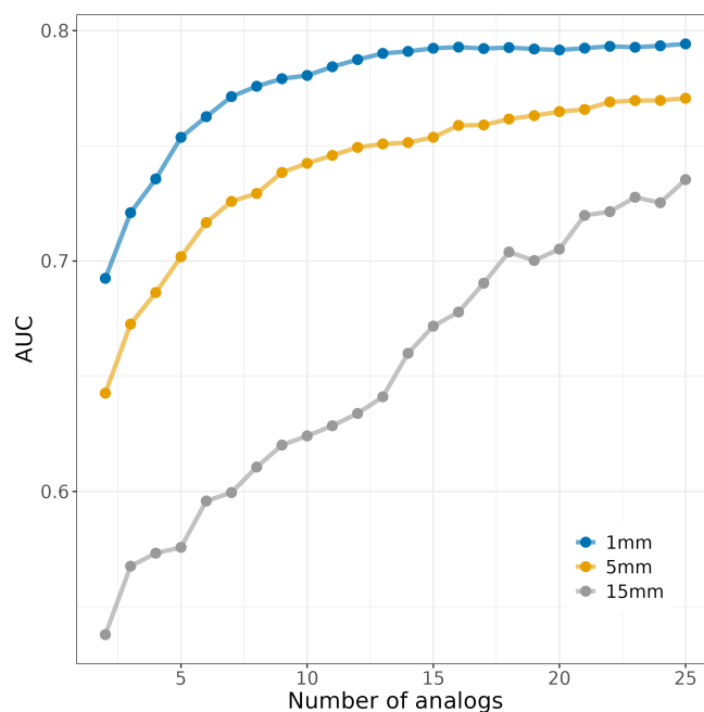
Figure 12. Evolution of AUC values based on the median with increasing number of ensemble members for the three considered event thresholds 1, 5 and 15 mm per 24 h for the 10-year period 1990–1999.
