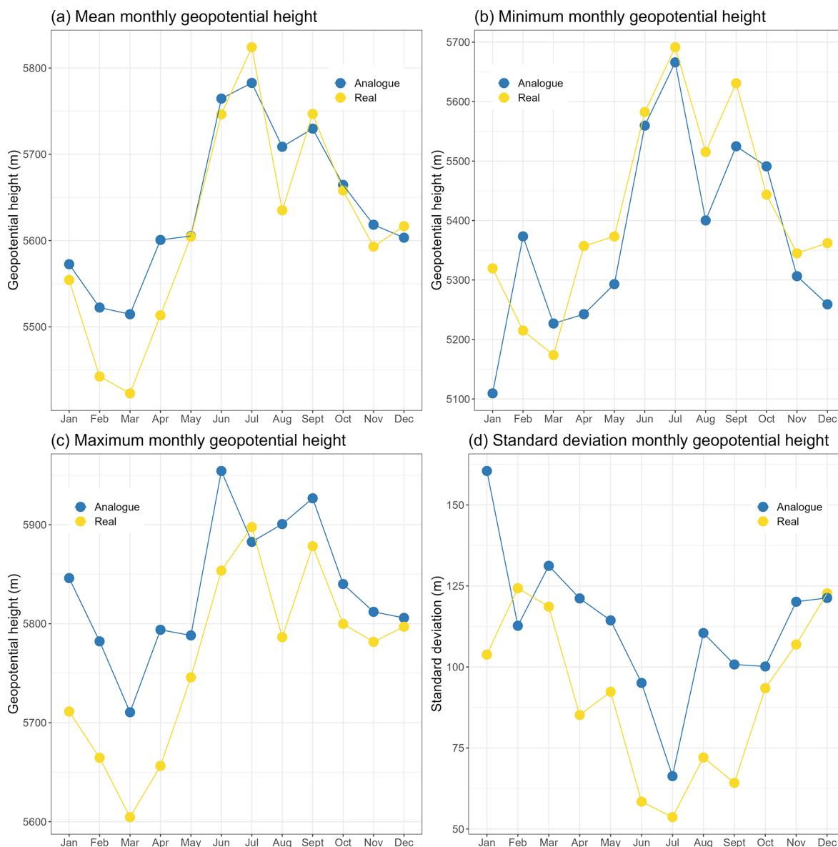
Figure 5. Monthly statistics of geopotential height at 500 hPa pressure level in Uccle at 12:00 UT in 2006. Top left to bottom right: (a) mean, (b) minimum, (c) maximum and (d) standard deviation. The general pattern between real and analog days seems similar across all four summary measures.
