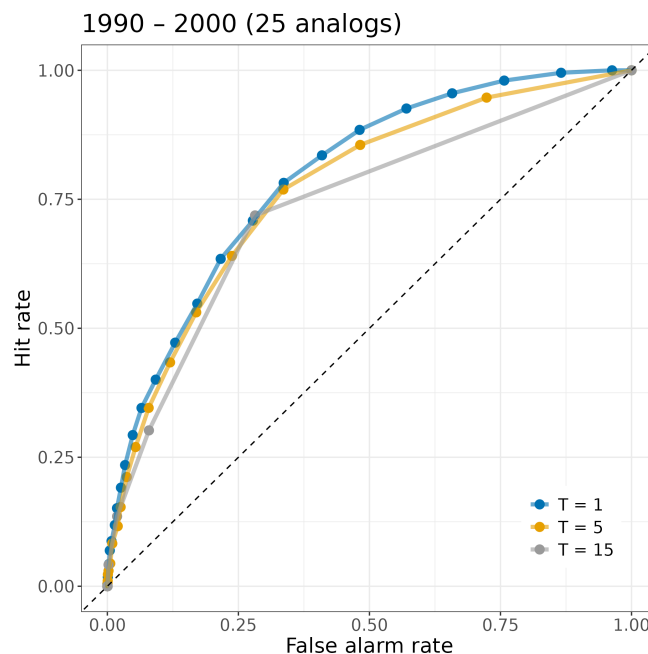
Figure 11. Examples of ROC curves for common and rare events during the 10-year period 1990–2000 for 25 analogs. ROC curves and corresponding AUCs for precipitation forecasts with event thresholds: 1, 5, and 15 mm per 24 h (1990–1999, 25-member ensemble).
