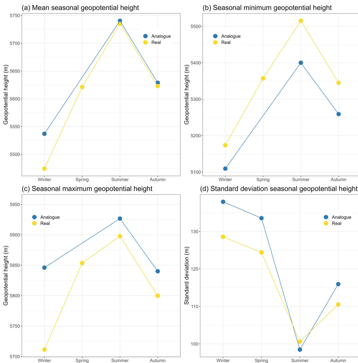
Figure 6. Seasonal statistics of geopotential height at 500 hPa in Uccle at 12:00 UT in 2006. Top left to bottom right: (a) mean, (b) minimum, (c) maximum and (d) standard deviation. The general pattern seems similar in the different cases.
