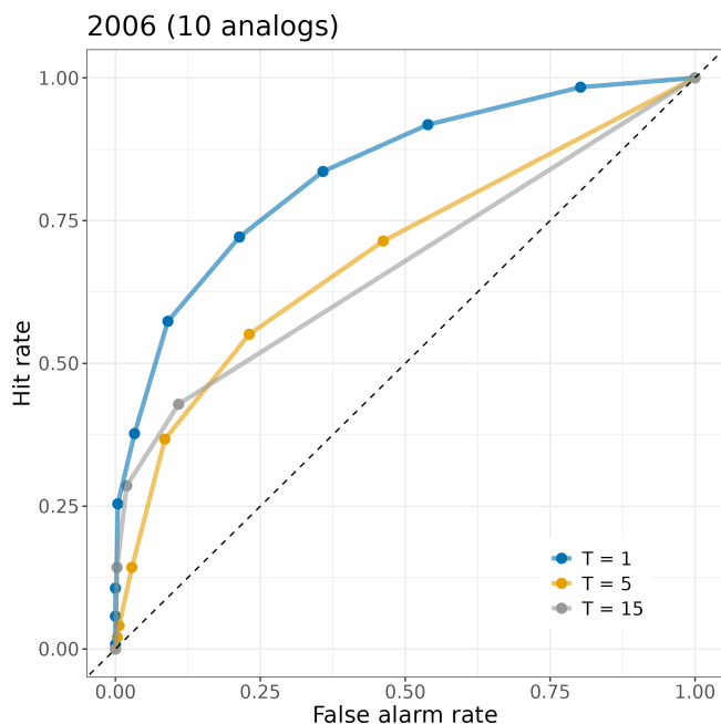
Figure 9. Examples of ROC curves for common and rare events. ROC curves and corresponding AUCs for precipitation forecasts with event thresholds: 1, 5, and 15 mm per 24 h (2006, 10-member ensemble).
