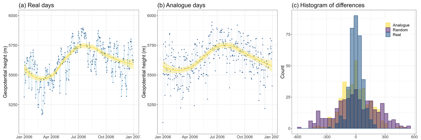
Figure 4. The temporal evolution in geopotential height at the 500 hPa pressure level at 12:00 UT in Uccle in 2006 (a); the corresponding data on the best analog days in 2006 (b); differences in geopotential height on analog days, real days and random days (c). The yellow curves in the first two plots aid the eye in seeing patterns in the presence of overplotting by fitting a smooth curve to the data.
