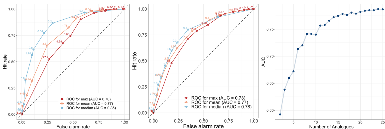
Figure 8. From left to right: ROC curve for Uccle for 2006 for models based on different summary statistics using the 10 best analogs; ROC curve for Uccle for the period 1990–1999 for models based on different summary statistics using the 10 best analogs; The evolution of AUC values in relation to the increasing number of analog days per target day in 1990–1999, using the median as the predictive measure.
