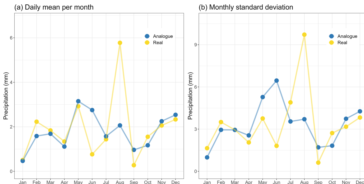
Figure 7. Evolution of (a) daily mean per month and (b) monthly standard deviation of 24 h precipitation accumulation in Uccle in 2006.
