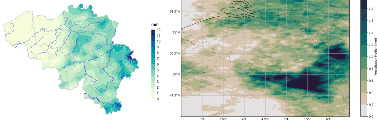
Figure 15. Comparison of observed daily precipitation accumulation on the left and the median accumulation derived from the 25 best analog days on the right.
