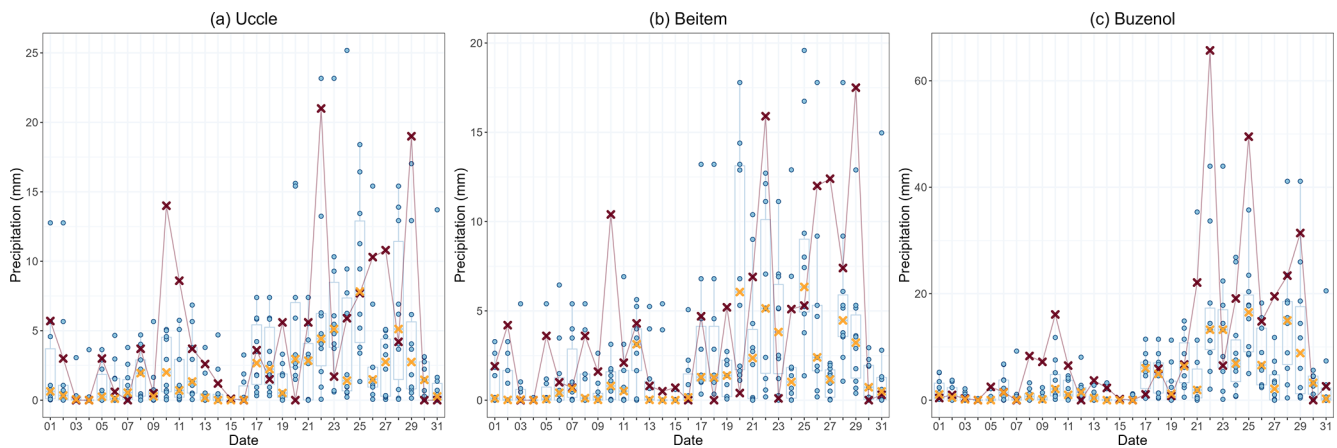
Figure 13. Daily precipitation accumulation patterns (distributions) for January 1995 using the ten most similar analog days using radar values indicated by the blue dots. The daily observations obtained from the pluviometer in (a) Uccle, (b) Beitem and (c) Buzenol indicated by the purple markers. The yellow crosses represent the median precipitation value for each day based on these 10 best analog days.
