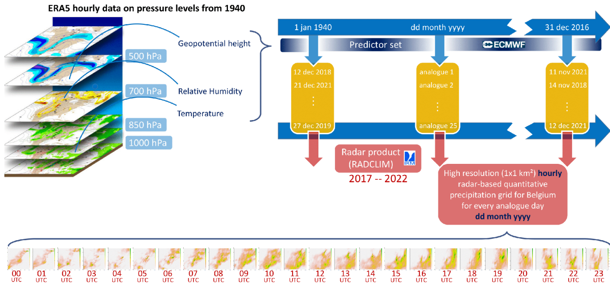
Figure 1. Overview figure illustrating the process of downscaling and validation of precipitation fields based on the analog method. The procedure in a nutshell: (i) selection of the analog days within the period covered by the radar based on large-scale fields of ERA5 to a specific target day in the past; (ii) association of the hourly precipitation fields of the analog days to the specific target in the past; (iii) construction of the best estimate of the precipitation field, either by using a single analog or a combination of them.
