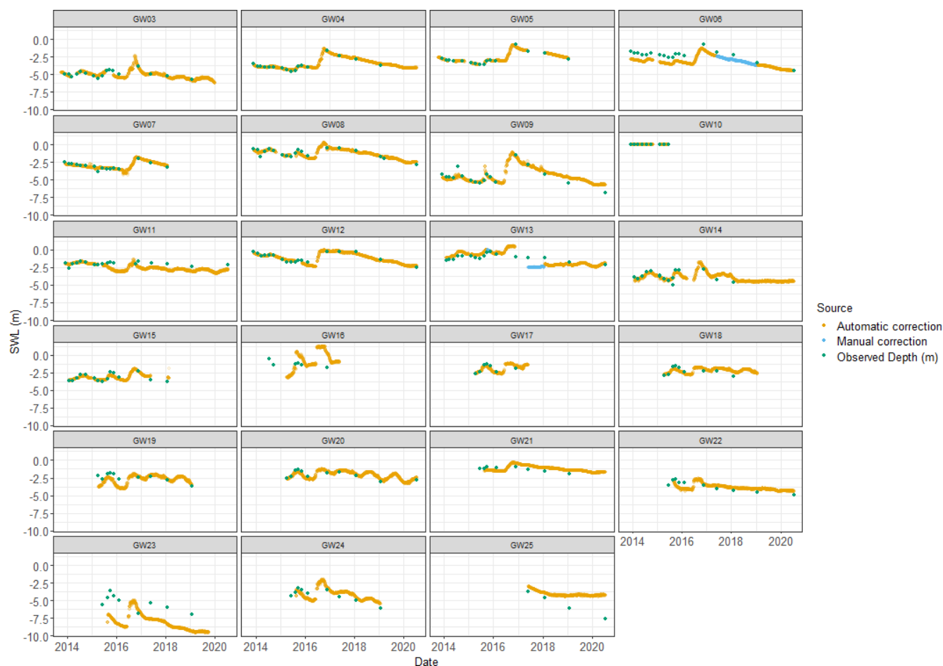
Figure 7. Overview of the corrected groundwater time series for all the wells. Different panels relate to the different locations highlighted in Fig. 2.
