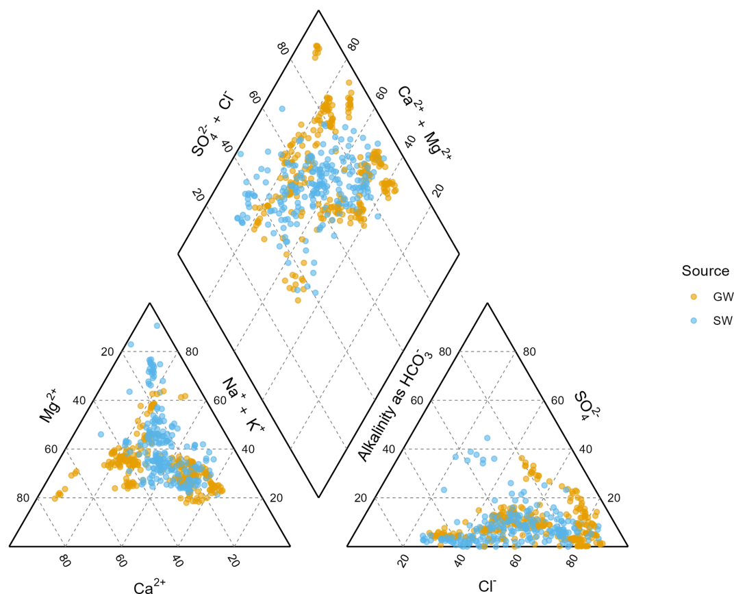
Figure 10. Piper-plot of all groundwater and surface water data collected over the period with complete major anion data.
