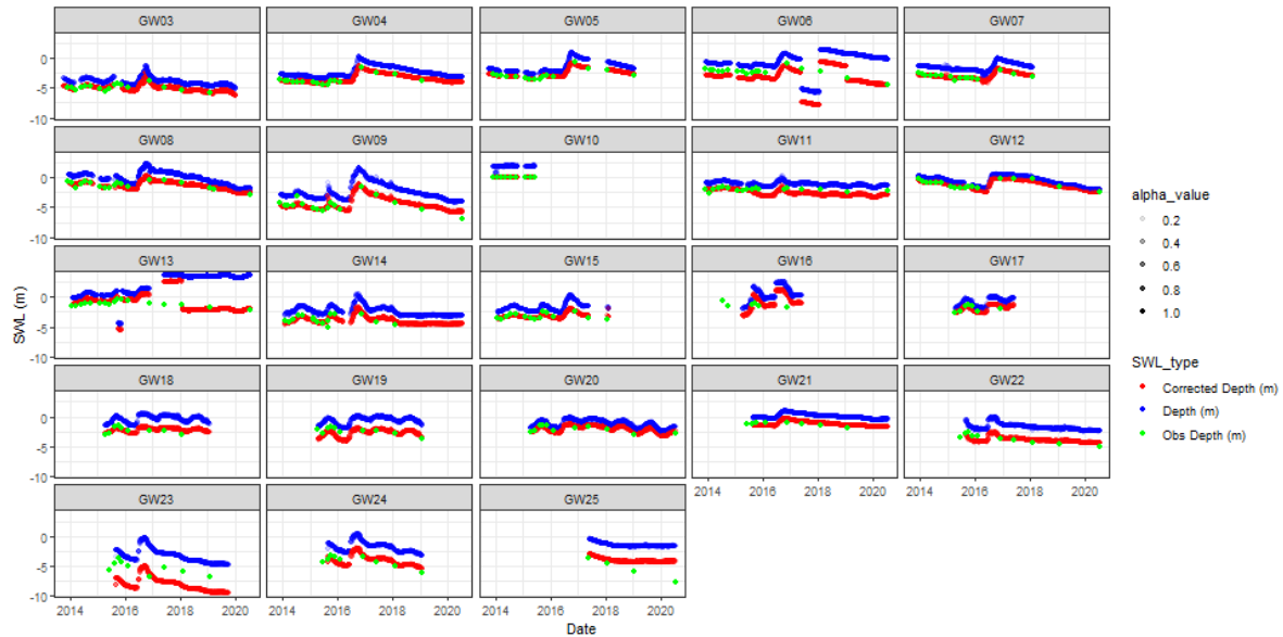
Figure S1: Groundwater level logger data corrected for cable length and automatically matched to observed data.
