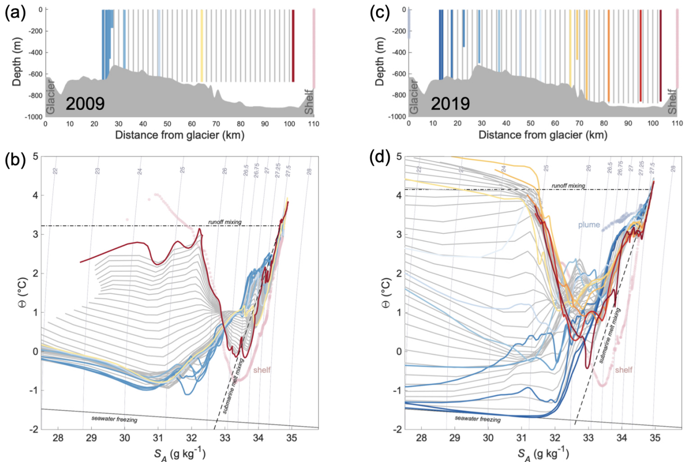
Figure 7. Comparisons of original profiles and gridded data for years 2009 ( a, b ) and 2019 ( c, d ) in \Theta – S_A diagrams ( b, d ). Panels ( a ) and ( c ) show the along-fjord location of the original profiles, colored by distance from the glacier, in comparison to location of the grid cells (grey lines). \Theta – S_A diagrams ( b, d ) show original profiles, colored by distance from the glacier in panels ( a ) and ( c ). Grey lines are the gridded data with every column in the grid plotted as an individual profile. Shelf profiles from both years are shown in light pink and two plume profiles from 2019 are shown in light blue. Mixing lines are plotted for submarine ice melt (dashed line) and melt runoff (dot-dash line) and the seawater freezing line is the black solid line. Grey contours are potential density anomaly isopycnals in \text{kg m}^{-3} .
