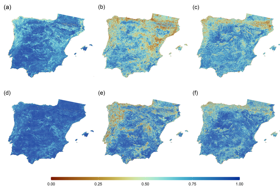
Figure 4. Spatial distribution of Willmott's d index for NDVI time-series harmonization, calculated per pixel. Panels (a)–(c) show the AVHRR–MODIS harmonization: (a) overall annual agreement, (b) 1 December semi-monthly period, and (c) 1 June semi-monthly period. Panels (d)–(f) show the AVHRR–MODIS–VIIRS harmonization: (d) overall annual agreement, (e) 1 December semi-monthly period, and (f) 1 June semi-monthly period.
