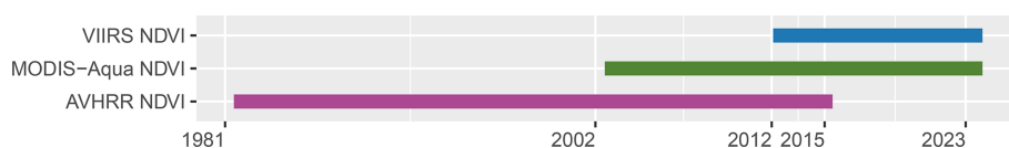
Figure 1. Temporal cover of the AVHRR, MODIS, and VIIRS NDVI datasets.
