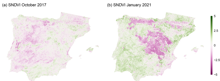
Figure 11. SNDVI from significant climatic events. Panel (a) shows the impact of the severe drought and wildfires on the Iberian Peninsula in October 2017, with notable vegetation stress indicated by standard deviation values below -3 . Panel (b) presents SNDVI from the storm Filomena in January 2021, highlighting areas with unprecedented snowfall.
