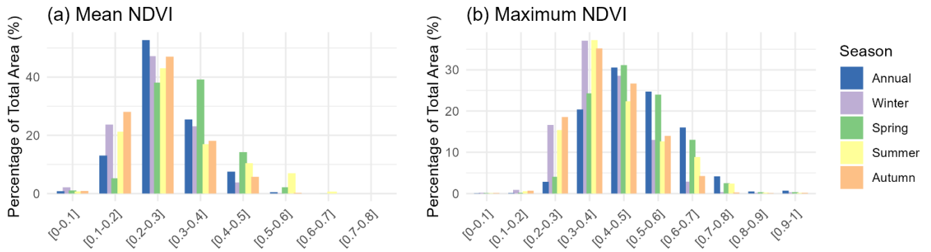
Figure S4. Annual and seasonal distribution of NDVI values across the Iberian Peninsula and Balearic Islands. (a) The mean NDVI distribution presents the average vegetation cover per NDVI interval for each season and annually for the time-series (b) The maximum NDVI distribution highlights the peak vegetation cover within each NDVI interval, also segmented by season and annually. Each bar represents the percentage of the total area falling within specific NDVI ranges, demonstrating seasonal variation in vegetation activity.
