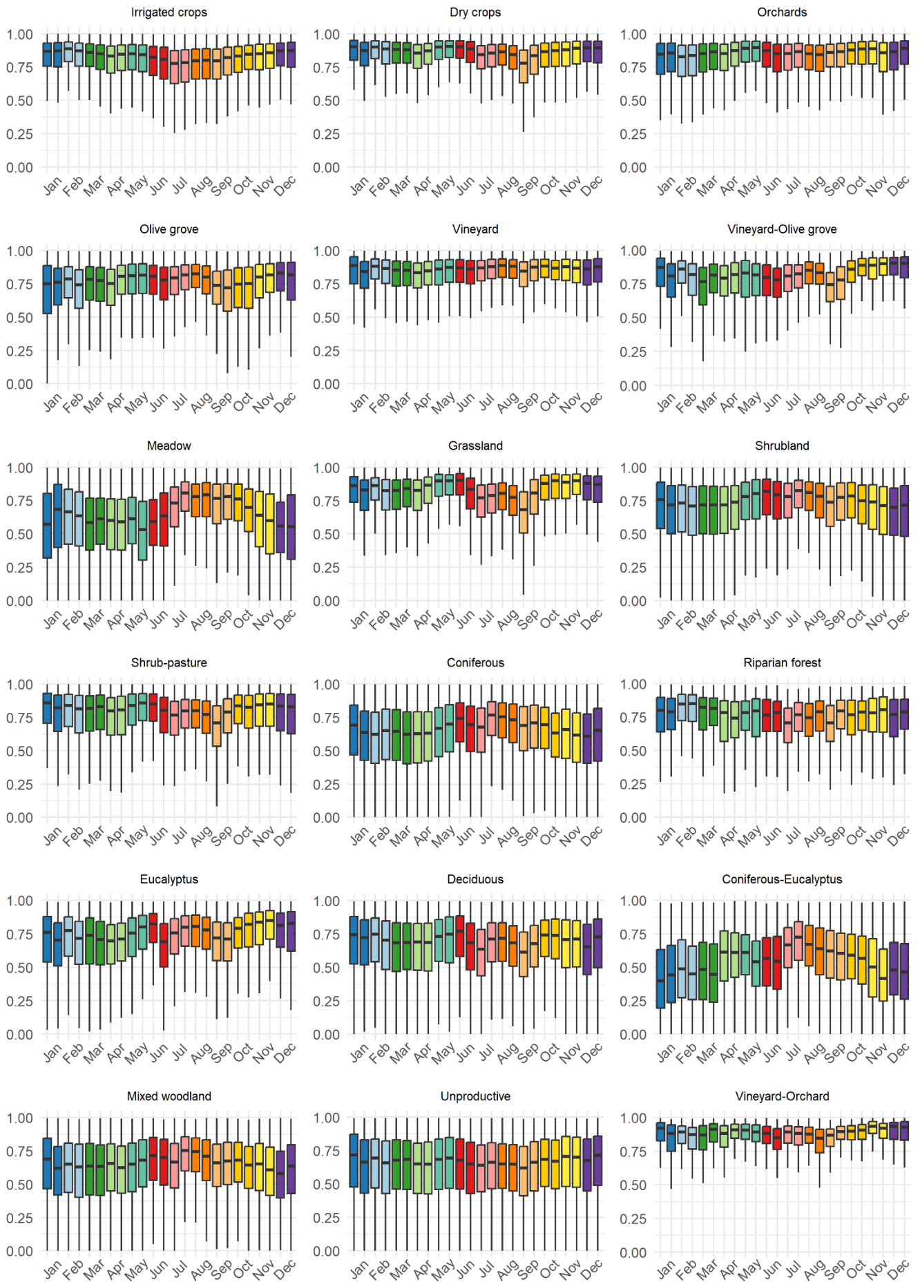
Figure S3. Distribution of Willmott's d index values by land cover and semi-monthly periods between harmonized AVHRR-MODIS-VIIRS vs VIIRS original data.
