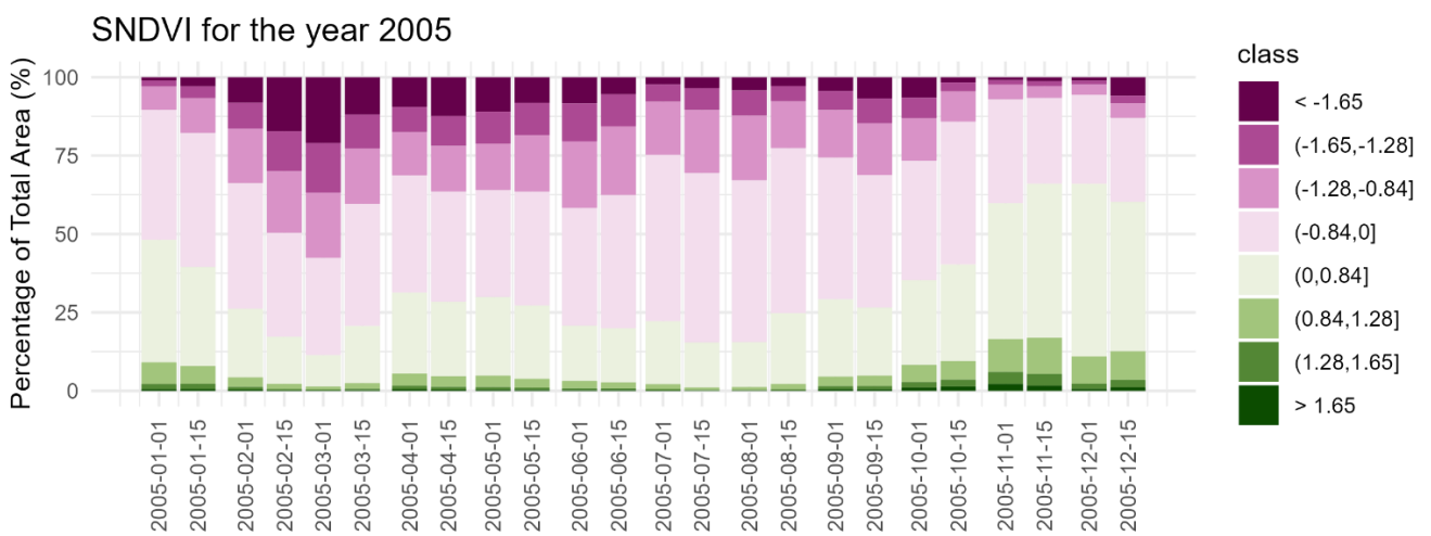
Figure S5. Temporal evolution of vegetation anomalies (SNDVI) for the year 2005 in the Iberian Peninsula and Balearic Islands. The color gradient from purple to dark green marks the range of SNDVI values, with purple representing the lowest (< -1.65) and dark green the highest (> 1.65), capturing vegetation dynamics during the 2005's drought event.
