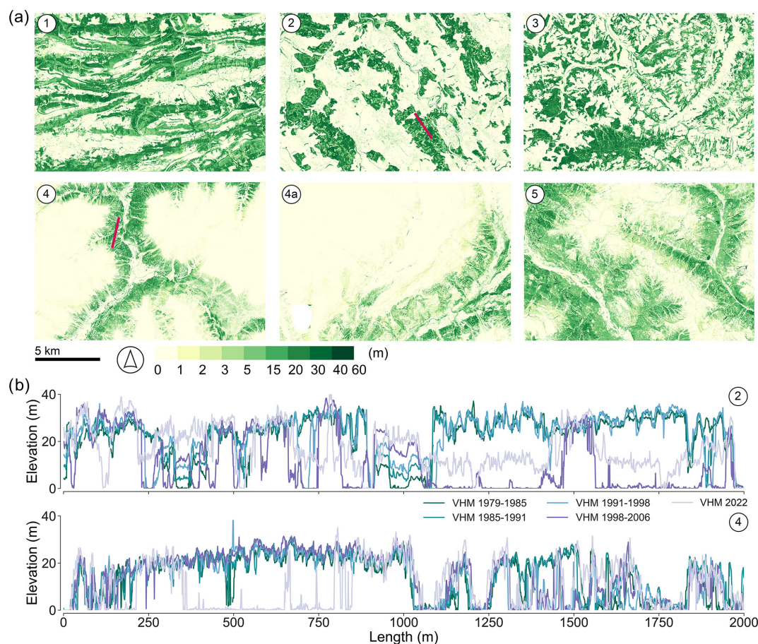
Figure 10. Illustration of (a) the vegetation height models (VHM) of epoch 2 (1985–1991) for the six selected study sites. The VHM correspond to the years 1987 for site 1, 1988 for site 2, 1986 for sites 3 and 4a, 1991 for sites 4, and 1989 for site 5. (b) The profile of the VHM from historical aerial images for the four epochs and from a modern airborne survey (2022) for study sites 2 and 4. The 2 km profile line is shown in red in (a).
