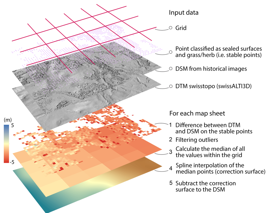
Figure 4. Illustration of the workflow to correct the elevation bias in the historical digital surface models (DSMs) for each map sheet. A correction surface is derived by a spline interpolation of the median height difference values (reference DTM – historical DSM at sample points “sealed surface” and “grass/herbs”) within regular grid cells (418 m).
