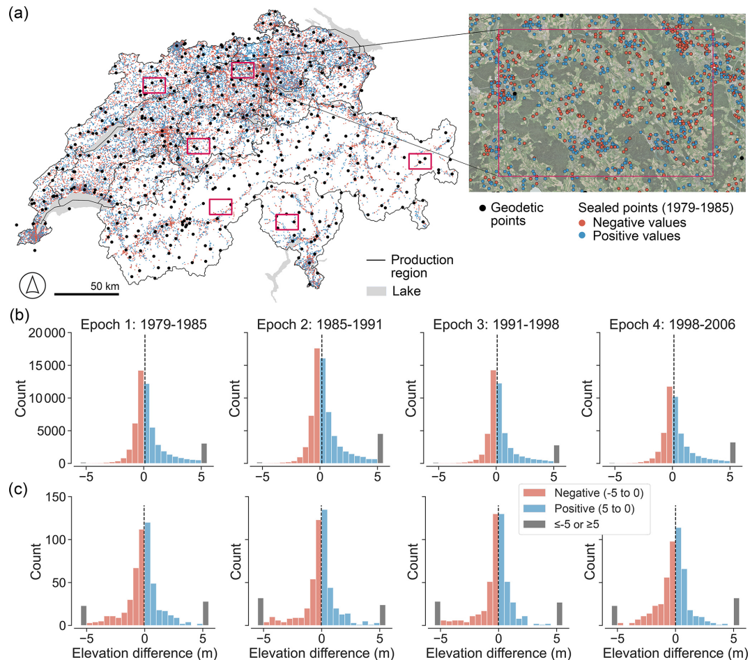
Figure 7. (a) Spatial distribution of the sealed surface points and the geodetic points used for the vertical accuracy assessment of the historical digital surface models (DSMs). Sealed surface points are depicted in blue and red, representing the positive and negative differences, respectively, between the DSM for epoch 1 and the reference digital terrain model (DTM, swissALTI3D). The inset shows the distribution of the sealed surface points and the geodetic points for study site 2, overlaid on the orthophoto for the year 2021 (swisstopo, 2023). Frequency distributions of the elevation difference in metres between the DSM and the DTM (b) on sealed surface points and (c) between the DSM and the geodetic points for the whole of Switzerland for the four epochs. The vertical dashed line indicates the median value. The bin size is 0.5 m. The histogram shows the distribution before the filtering used for the root mean square error (RMSE) calculation.
