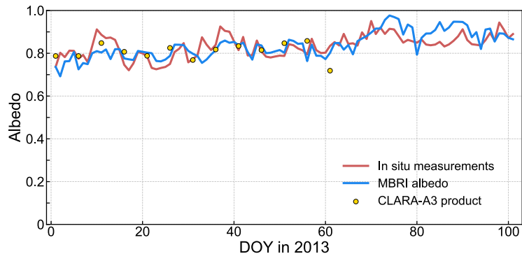
(b) Albedo at BSRN GVN
