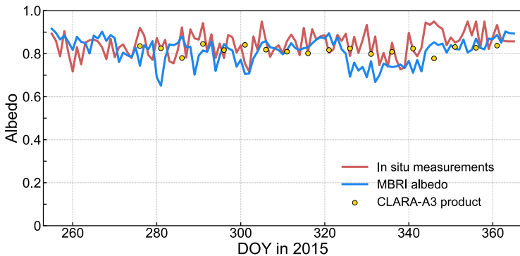
(c) Albedo at IMAU AWS17
