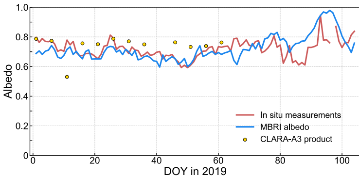
(a) Albedo at BSRN SYO
