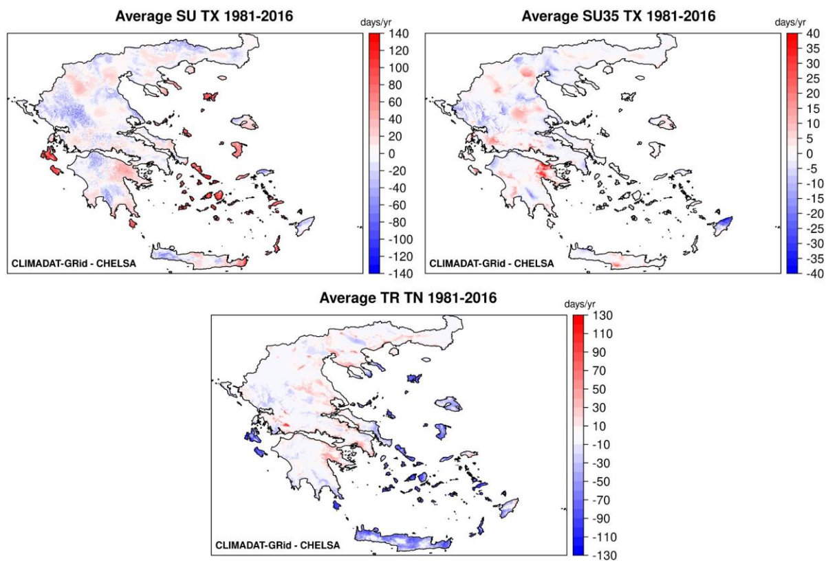
Figure S2. Average annual differences for SU, SU35 and TR between CLIMADAT-GRId and CHELSA for the period 1981–2016.
