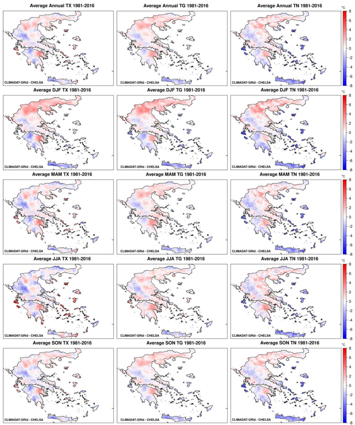
Figure S1. Average annual and seasonal differences for TX , TG and TN between CLIMADAT-Grid and CHLSA for the period 1981–2016.
