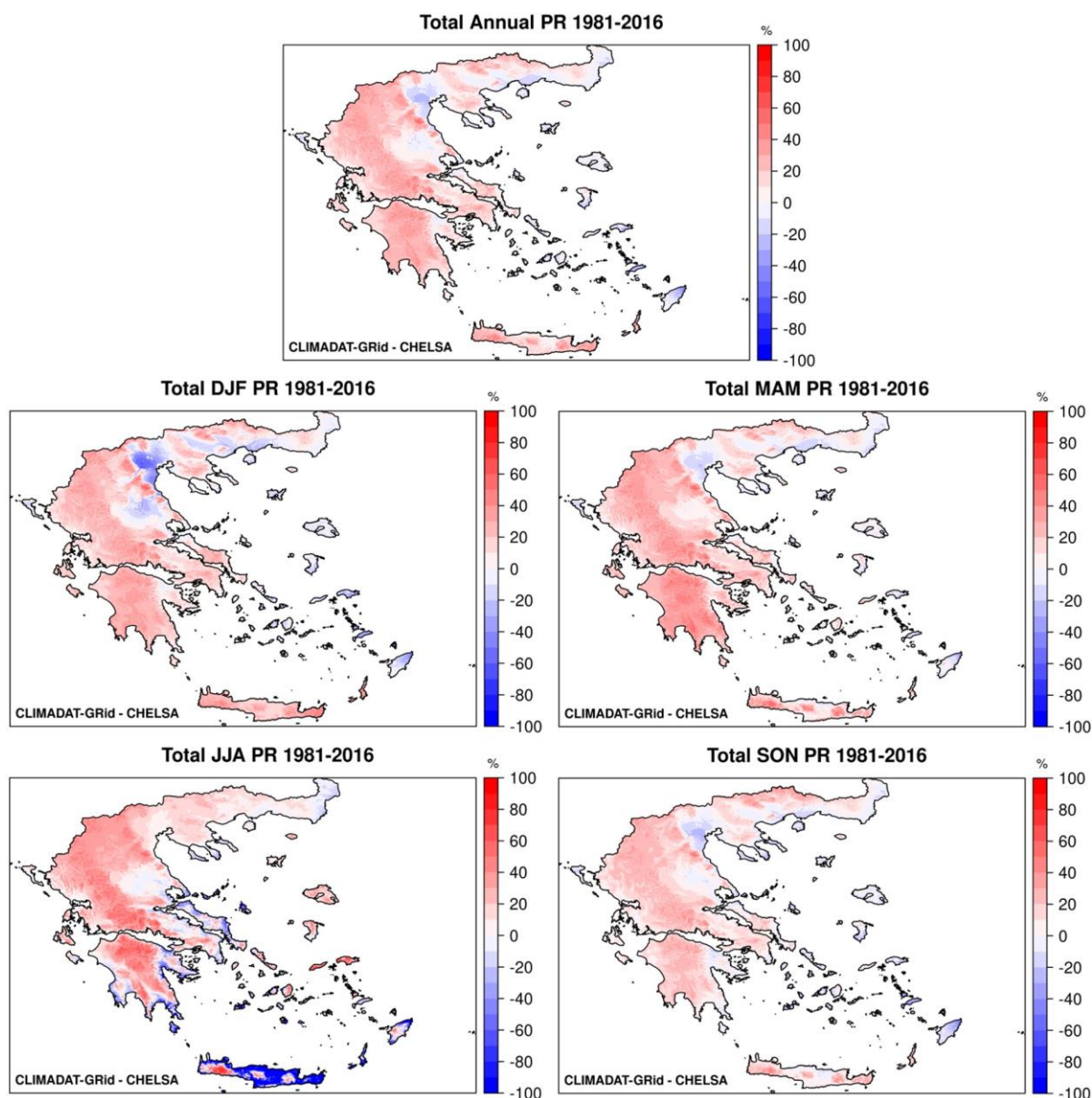
Figure S3. Average annual and seasonal relative differences in precipitation between CLIMADAT-GRid and CHELSA for the period 1981–2016.
