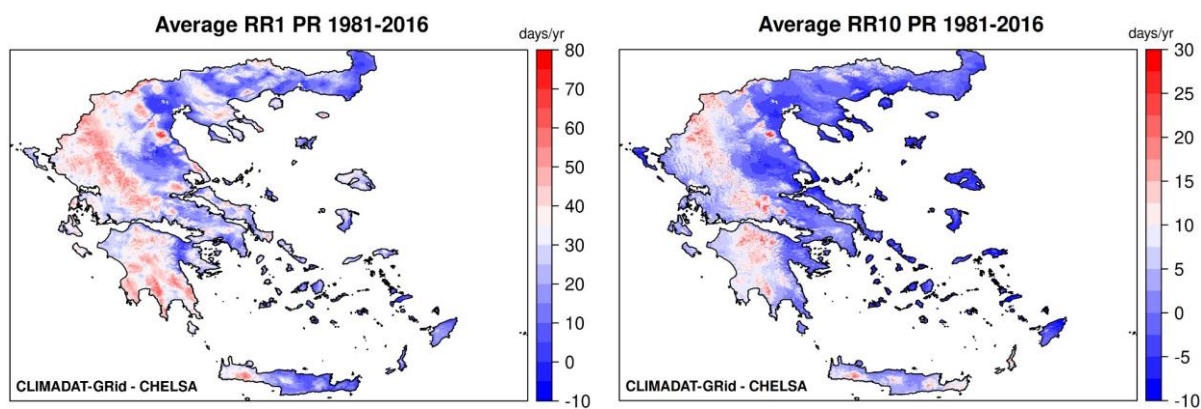
Figure S4. Average annual differences for RR1 and RR10 between CLIMADAT-GRid and CHELSA for the period 1981–2016.
