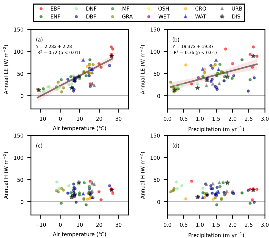
Figure 9. Relationships of annual energy fluxes of the latent heat flux ( LE ) ( a , b ) and sensible heat flux ( H ) ( c , d ) to the mean climate of the annual mean air temperature ( a , c ) and annual sum of the precipitation ( b , d ). The classification of the disturbed forest (DIS) is as in Fig. 8. Annual H values were calculated only for the case where there were no missing data in the mean seasonality, whereas the missing LE data during the winter were considered to be 0 for boreal forests in Russia. The lines represent linear regressions, with shading showing the confidence intervals ( p < 0.05 ), determined by excluding the data from DIS, urban areas (URB), and lakes and ponds (WAT). The values are shown in Table 3. Land cover type abbreviations are in Fig. 3.
