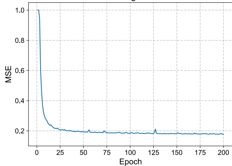
Training Loss
