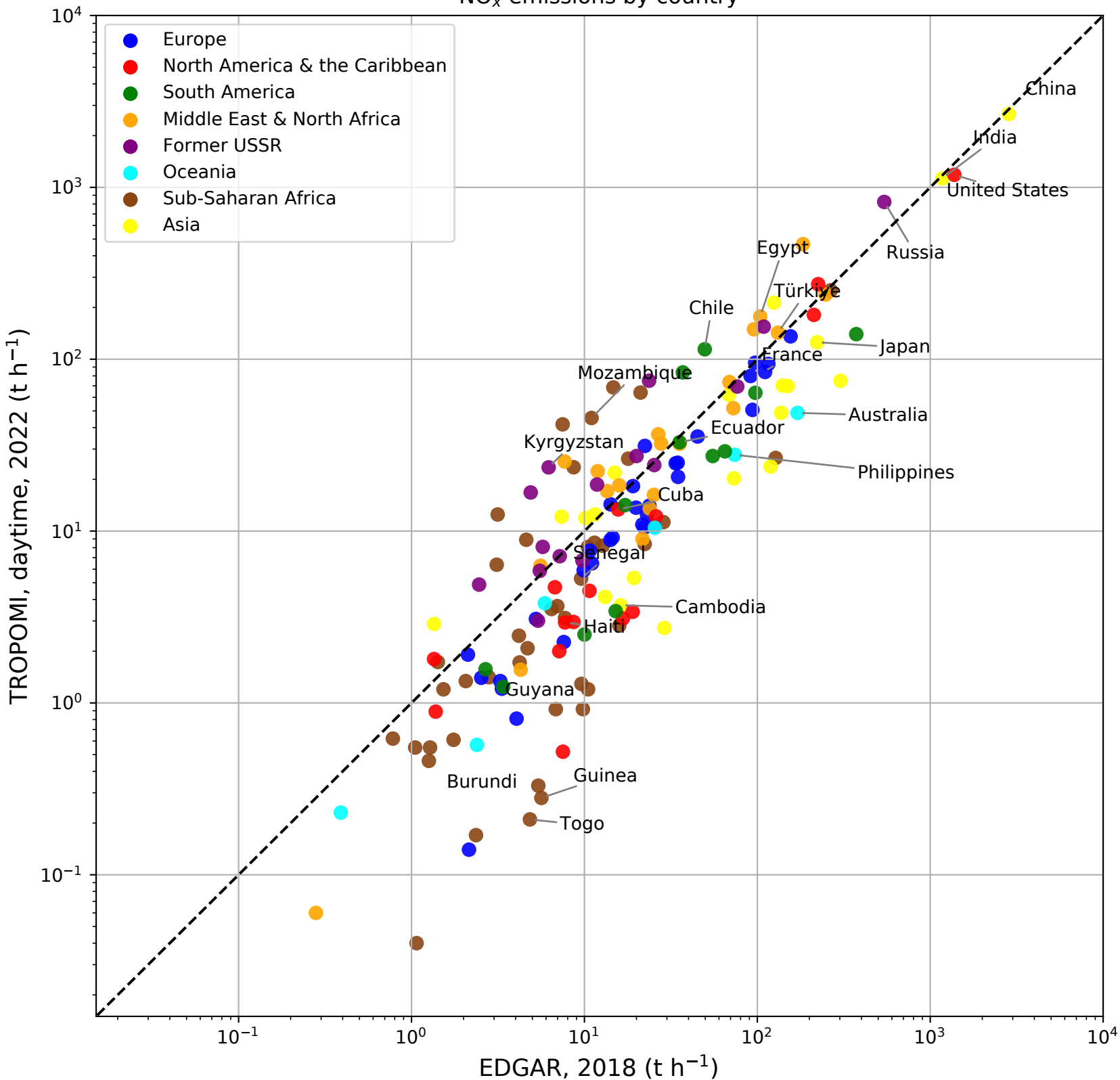
NO x emissions by country
