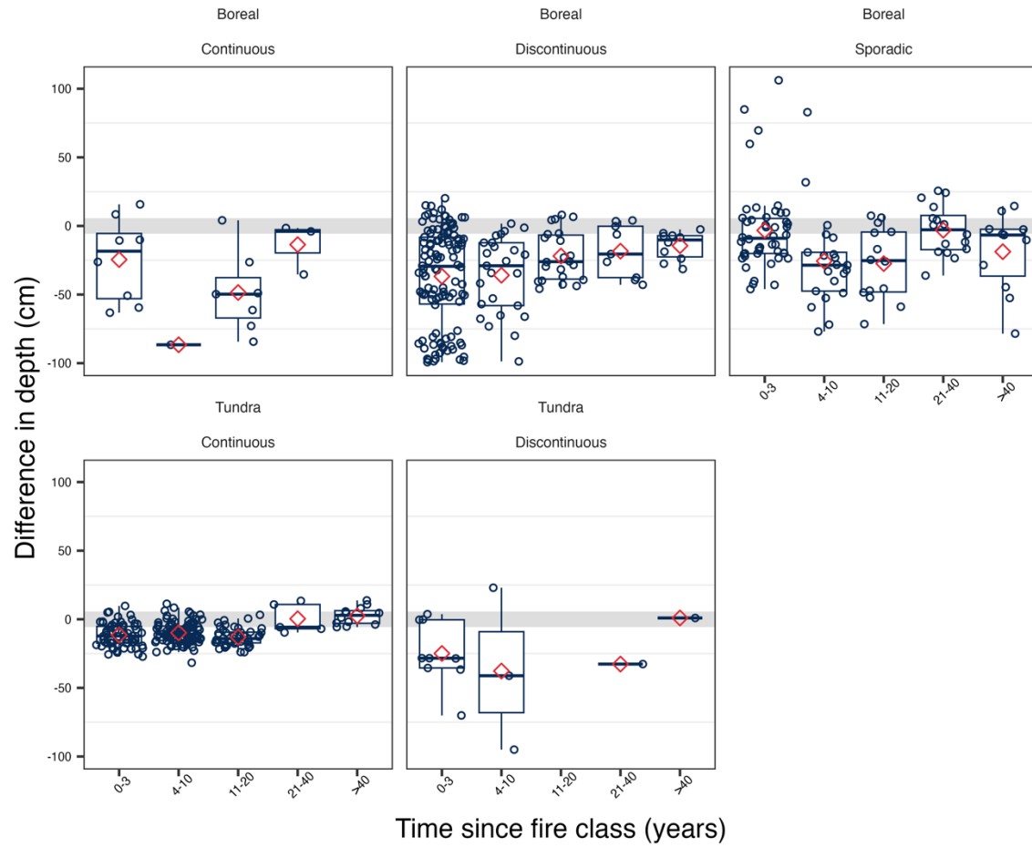
Figure S2. Boxplots of aggregated estimated ALT showing the difference in depth between burned and unburned sites by biome and permafrost extent. Individual estimated measurements were aggregated by pair identifier assigned by contributors. Points represent the difference between burned and unburned mean estimated ALT. The box and whisker plots show the quantiles with outliers as points and the red diamond indicates the mean.
