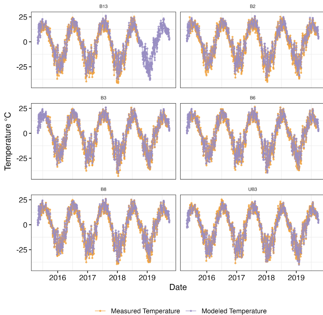
Figure S1. Daily air temperature between 2015 and 2019 from field measured and coarse resolution ERA5-Land data (modelled temperature) from six field sites in the Northwest Territories, Canada.
