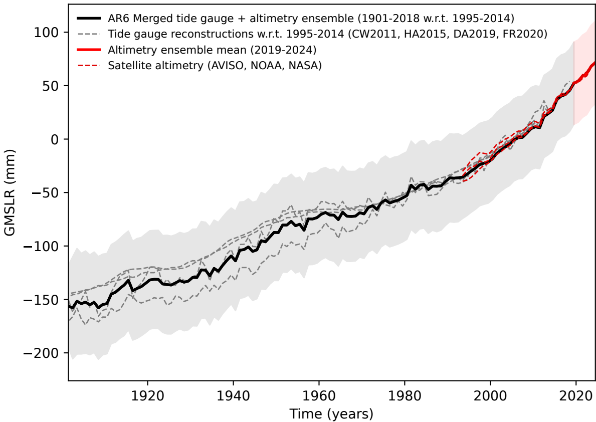
(a) Global mean sea-level rise
