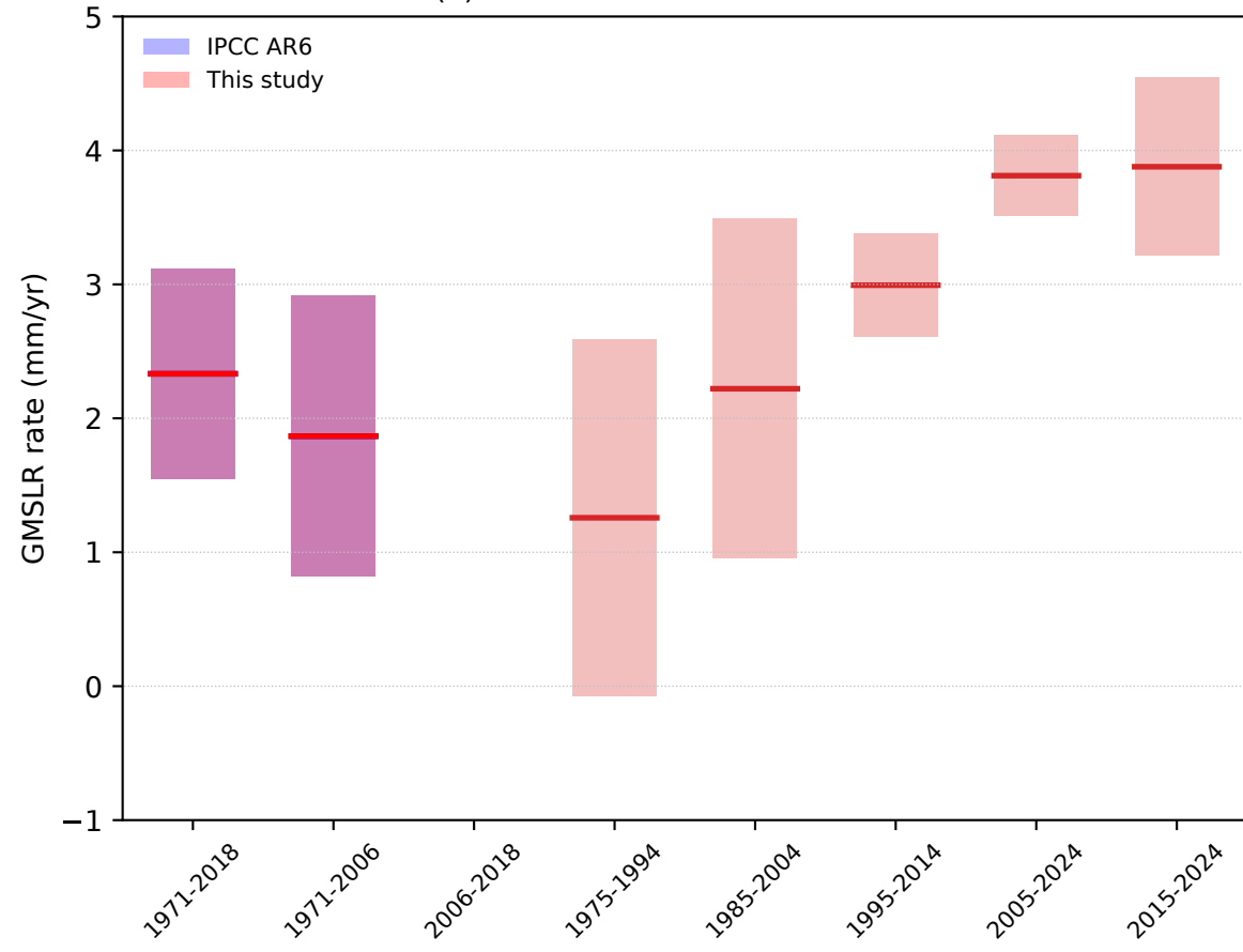
(b) Global mean sea-level rise rates
