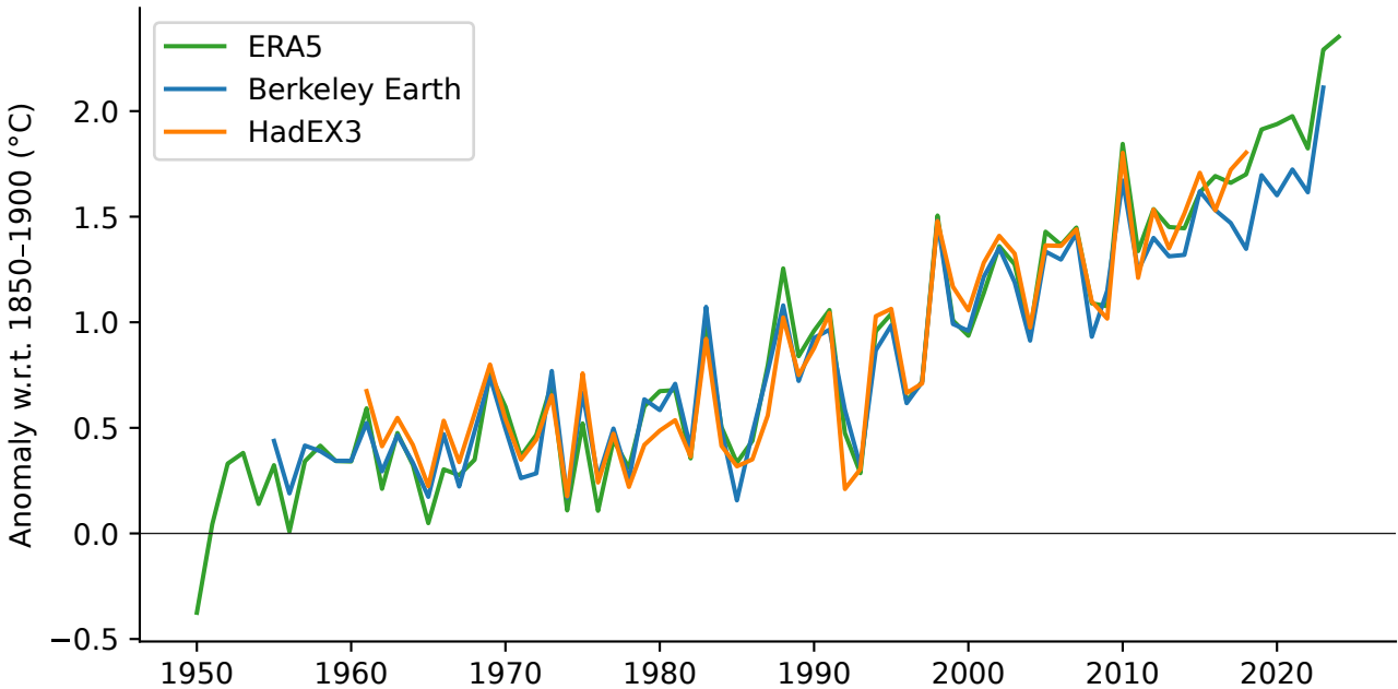
Land average annual maximum temperature anomaly
