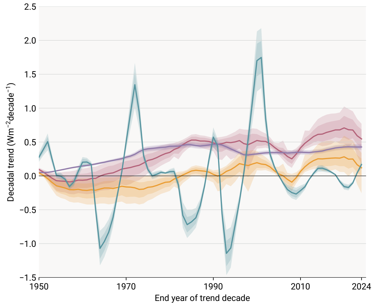
(a) Effective Radiative Forcing
