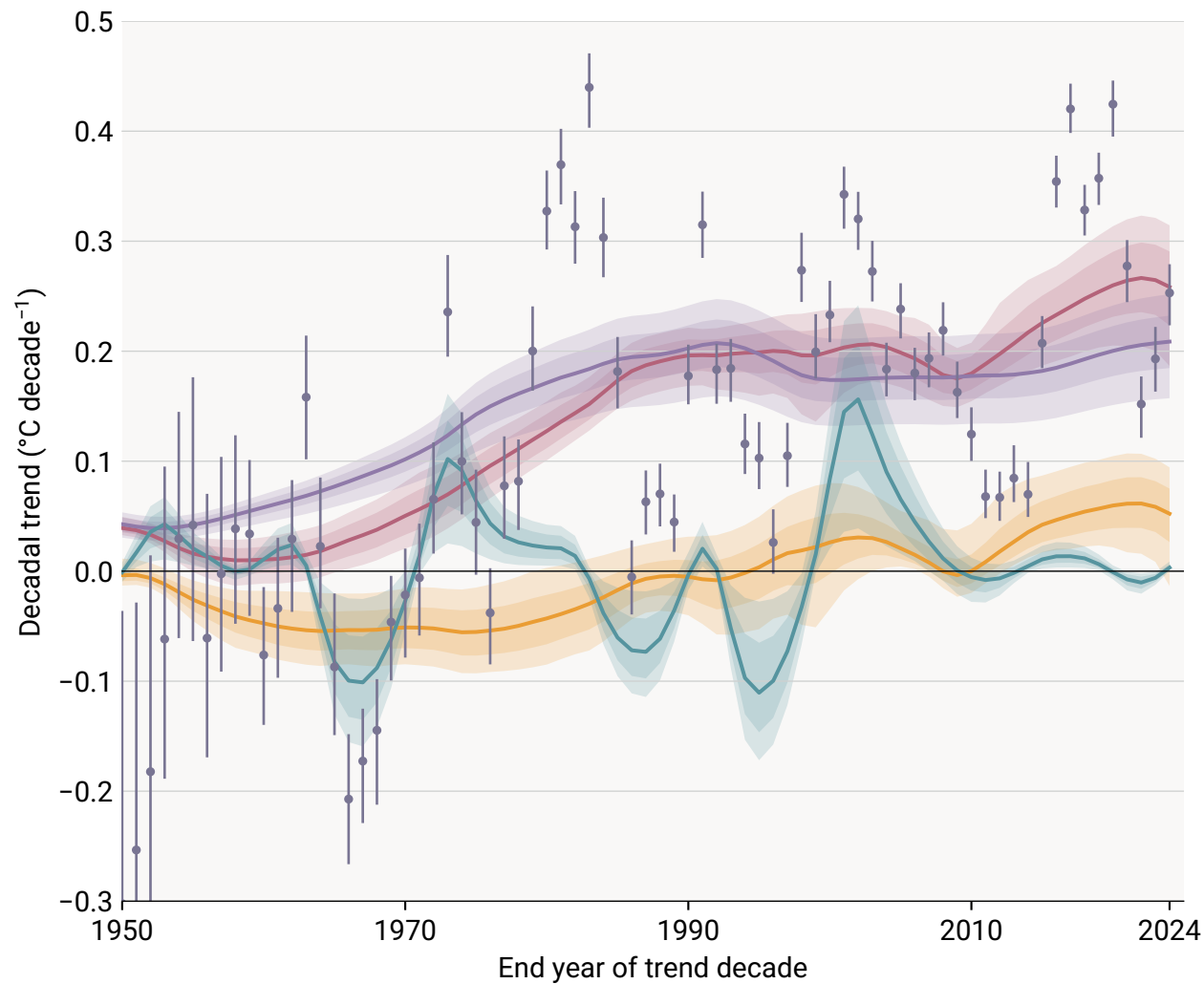
(a) Attributed Global Warming
