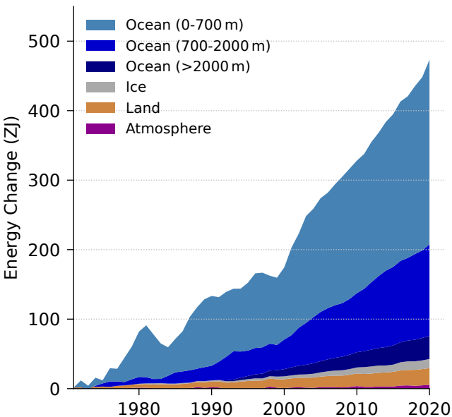
(a) Earth Heat Inventory
