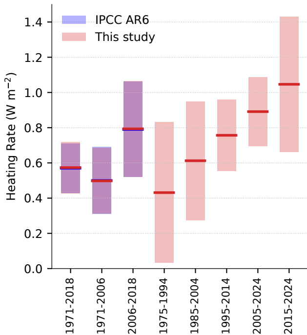
(b) Earth Energy Imbalance
