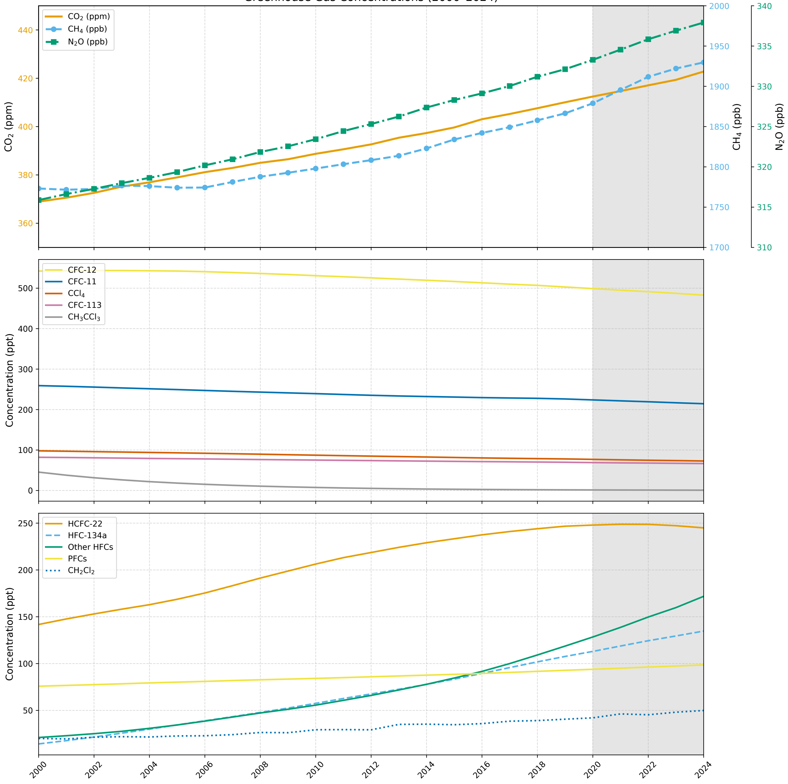
Greenhouse Gas Concentrations (2000-2024)
