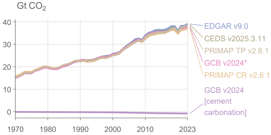
(b) Global CO 2 emissions from fossil fuel & industry (FFI)
