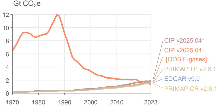
(f) Global F-gas emissions
