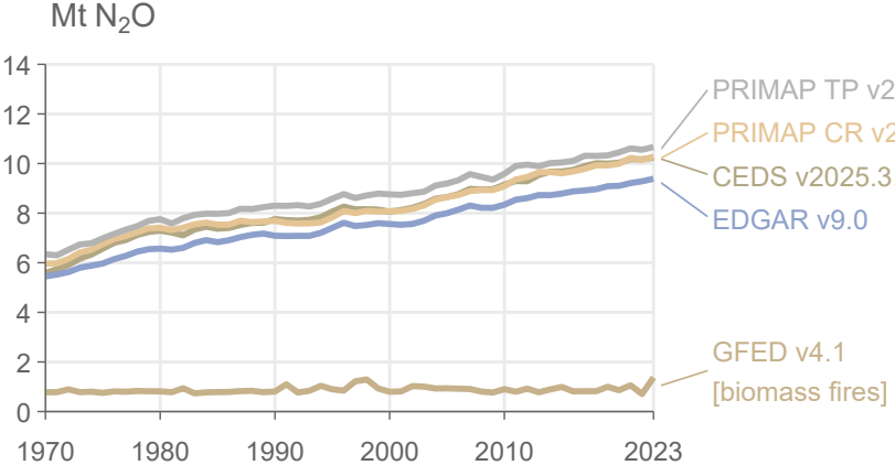
(e) Global N 2 O emissions
