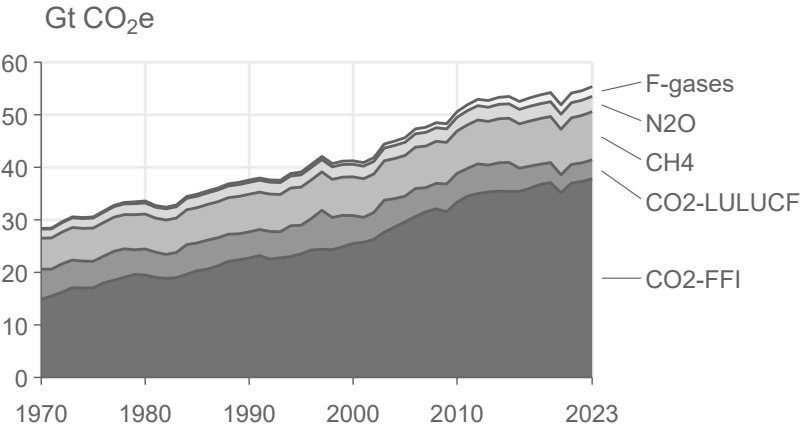
(a) Global total greenhouse gas emissions
