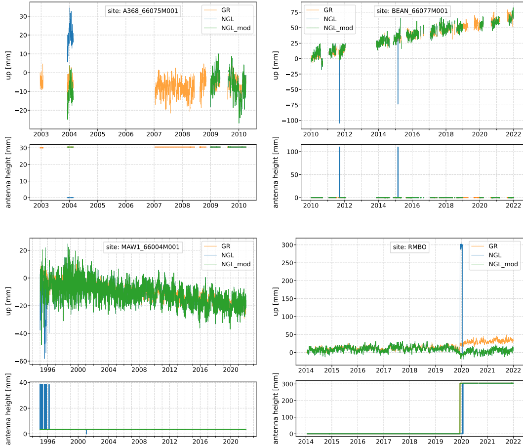
Figure S1. Time series of the vertical coordinate component from the GR (orange), NGL (blue) and NGL_mod with corrected antenna heights according to the GR meta data (green), together with the time series of antenna heights. The sites are selected to demonstrate the effect of false antenna height information on the coordinate trajectory, leading to errors in estimated rates (A368), single outliers (MAW1 and BEAN), or clustered outliers (RMBO).
