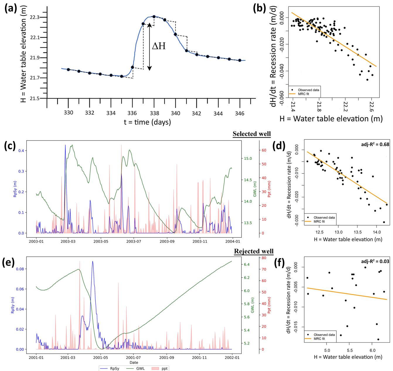
Figure 1. (a) Schematic representation of \Delta H evaluation in the WTF method, which is then used to obtain daily groundwater recharge using Eq. (1). (b) A typical dH/dt vs. H plot used to derive the MRC. The hydrographs in (c) and (e) show daily groundwater level (GWL, in m), precipitation (Ppt, in mm) and estimated recharge per unit specific yield ( RpSy , in m, discussed later) for a selected and a rejected well, respectively. Here, selection/rejection is based on representativeness of the MRC, which here is determined based on an adj-R^2 value of 0.2. Panels (d) and (f) show the dH/dt vs. H plot for the corresponding selected and rejected wells, respectively.
