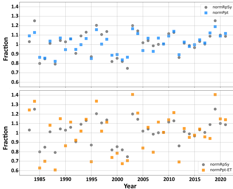
Figure 5. Inter-annual variation of normalized annual recharge (normRpSy, shown using solid grey dots), precipitation (normPpt, blue squares) and Ppt-ET (normPpt-ET, orange squares).
