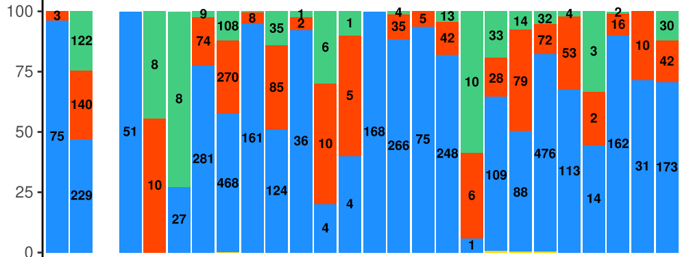
Minimum Temperature
