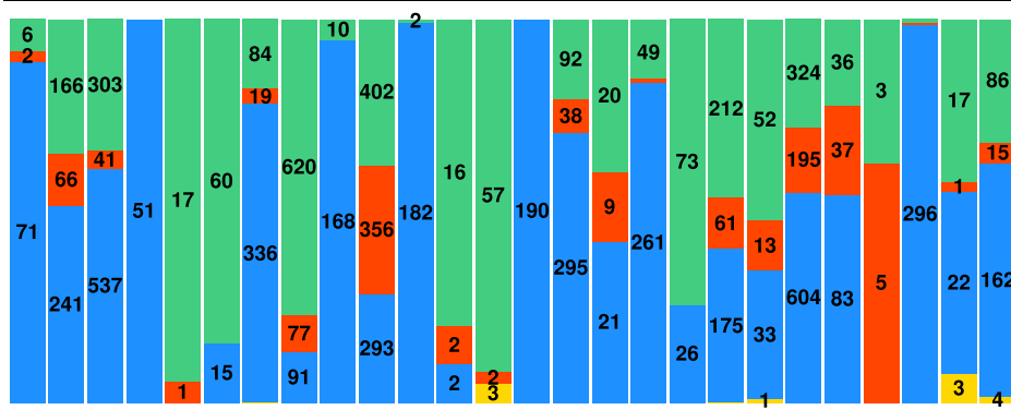
Precipitation
