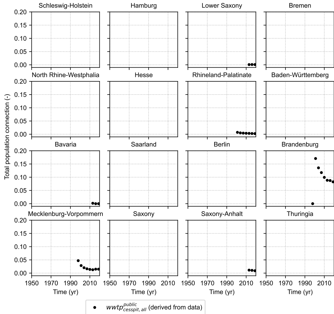
Figure S17. Data of resident population connected to WWTPs via cesspits for each NUTS-1 region ( wwtp_{cesspit,all} ). Source of the data: the data shown in this figure build on statistical data that mostly come from the Statistical Office of Germany and the different federal states, as well as additional sources, as detailed in Tables S11–S26. As explained in these tables, wwtp_{cesspit} is not always directly provided in the statistical reports, but is sometimes estimated in this study.
