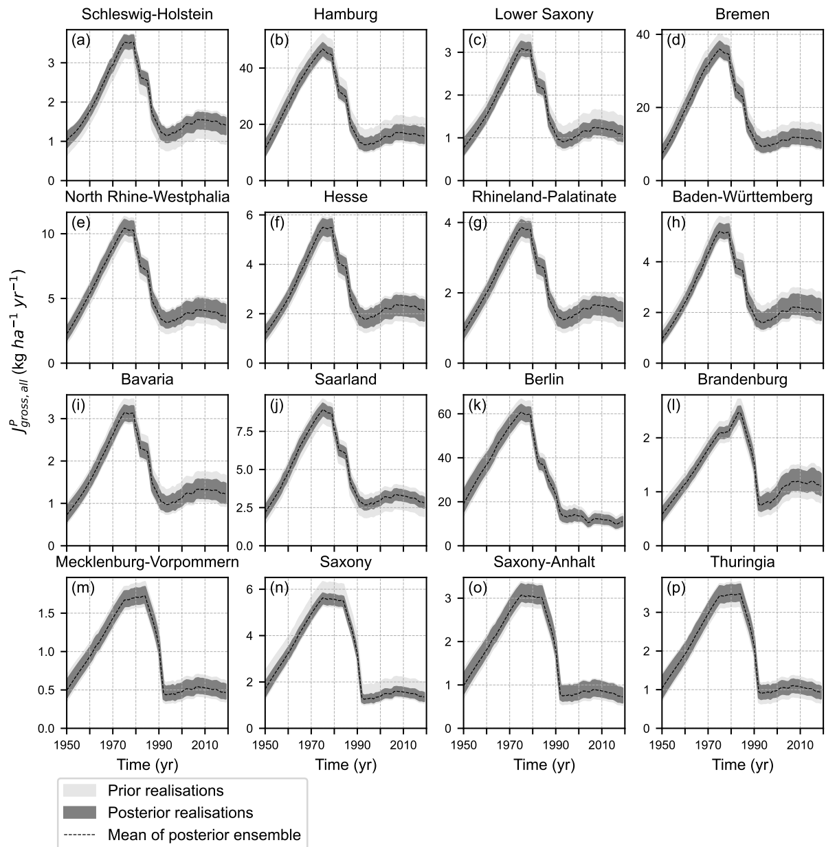
Figure S54. P gross emissions J_{gross,all}^P , including both the urban and rural components, and the domestic and industrial/commercial components, from the prior and posterior model realisations at NUTS-1 level for the period 1950–2019. The shaded areas delineate the minimum and maximum values of the 100,000 prior realisations (light grey) and the 100 posterior realisations (dark grey). © Authors 2024. This figure is distributed under a CC BY-NC-SA 4.0 License.
