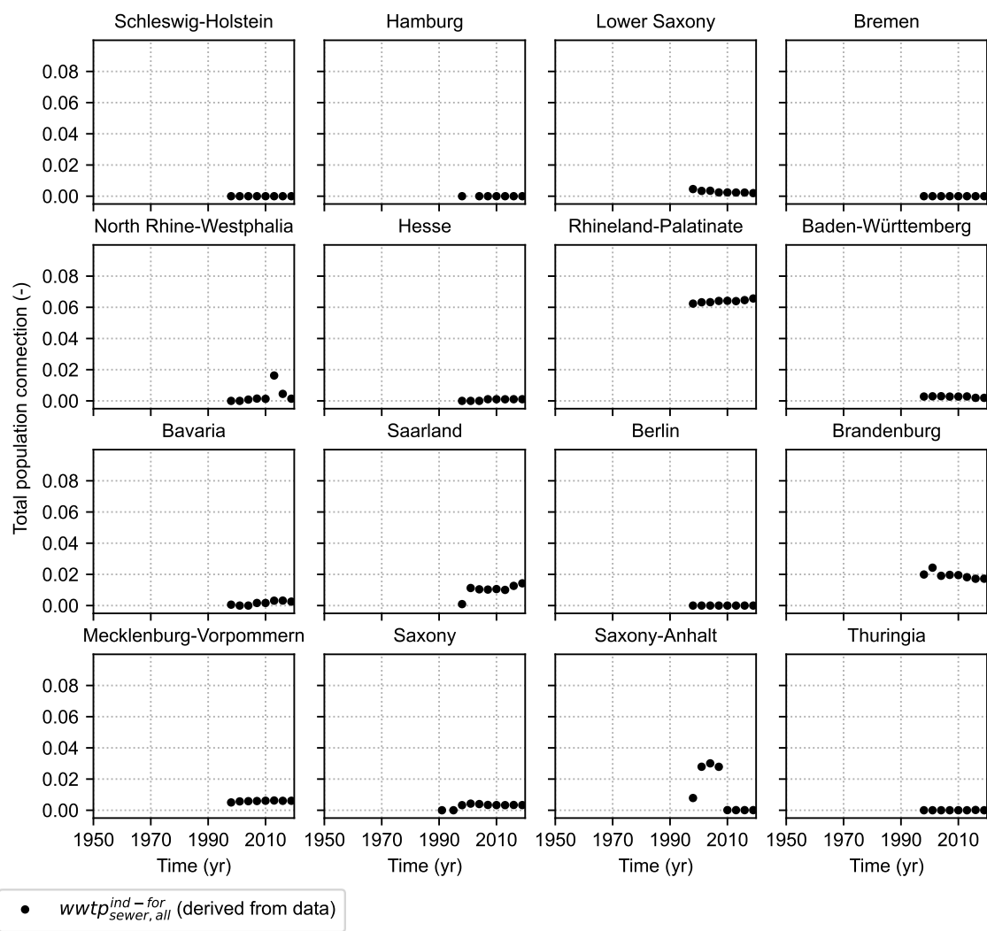
Figure S16. Data of resident population connected to industrial and foreign WWTPs for each NUTS-1 region ( wwtp_{sewer,all}^{ind-for} ). Data of population connection to industrial and foreign WWTPs are explicitly provided for the period 1998–2019, while before it is not explicitly reported whether WWTP connection data also account for industrial and foreign WWTPs in addition to public WWTPs. From the figure, we see that the percentage of population connected to industrial and foreign WWTPs is limited, since it is always lower than 3 %, apart from the state of Rhineland-Palatinate where it is around 6.5 %. Source of the data: the data shown in this figure build on statistical data that mostly come from the Statistical Office of Germany and the different federal states, as well as additional sources, as detailed in Tables S11–S26.
