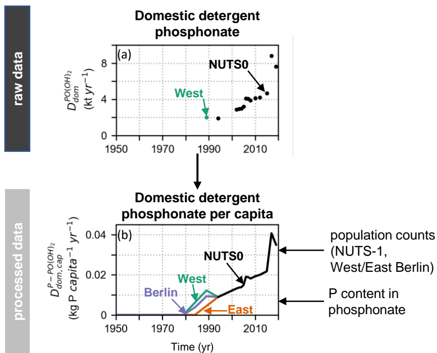
Figure S14. Raw (a) and processed (b) detergent phosphonate data for the domestic sector. © Authors 2024. This figure is distributed under a CC BY-NC-SA 4.0 License. Data source: (a) Raw data (domestic detergent phosphonate, DD_{dom}^{PO(OH)_2} ) come from ©IKW (2005, 2011, 2017, 2019) (license that does not allow commercial use at https://www.ikw.org/impressum ) and are provided for West Germany in 1989 and for Germany at NUTS-0 level for the period 1994-2019. (b) processed data for West, East and Berlin (domestic detergent phosphonate P per capita, D_{dom, cap}^{P-PO(OH)_2} ) build on the IKW data in (a), NUTS-1 level population data from the German Statistical Office and population data for West/East Berlin from the Statistical Office of Berlin (details on population data sources in Table 2 in the main text).
