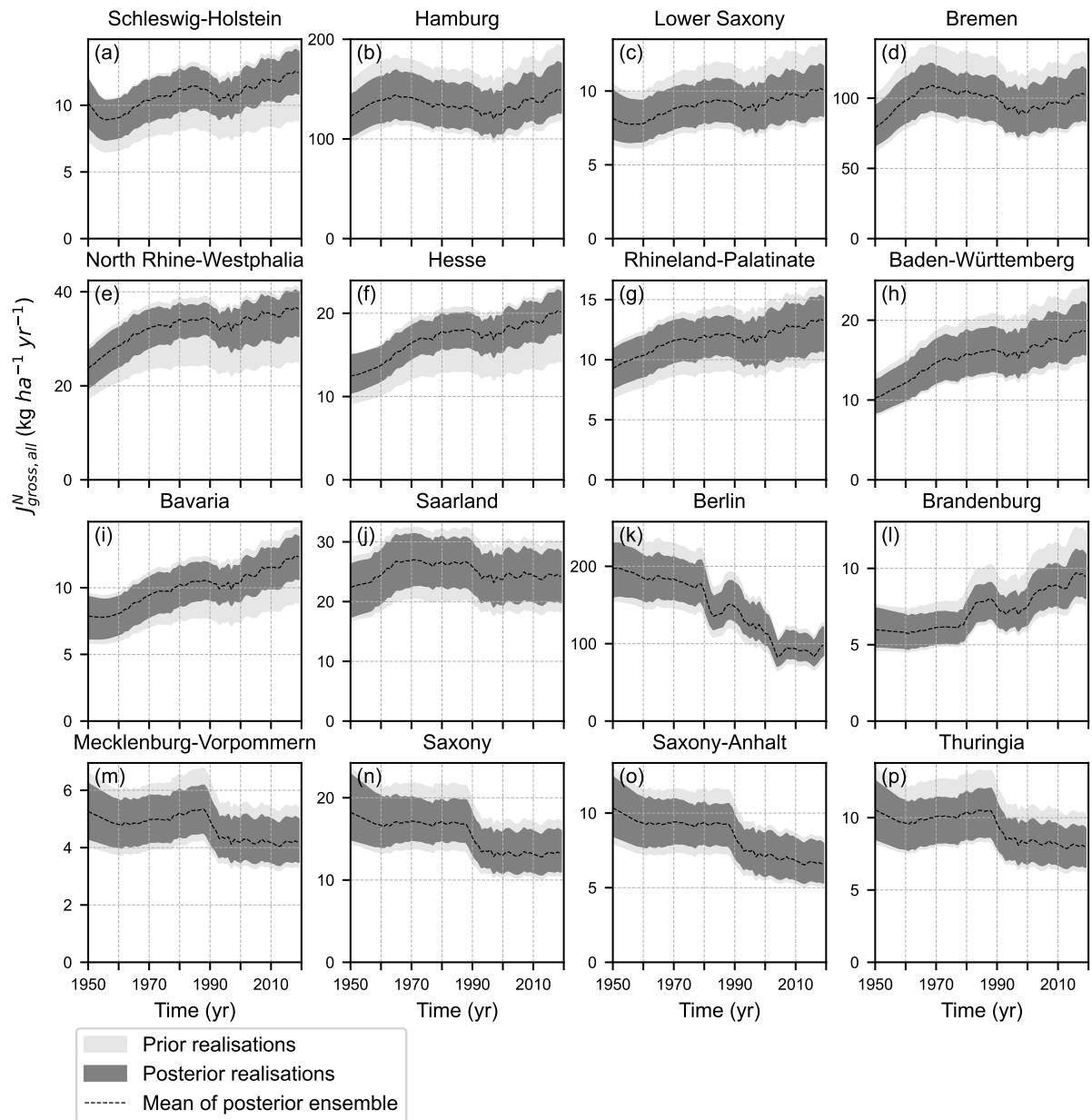
Figure S53. N gross emissions J_{gross,all}^N , including both the urban and rural components, and the domestic and industrial/commercial components, from the prior and posterior model realisations at NUTS-1 level for the period 1950–2019. The shaded areas delineate the minimum and maximum values of the 100,000 prior realisations (light grey) and the 100 posterior realisations (dark grey). © Authors 2024. This figure is distributed under a CC BY-NC-SA 4.0 License.
