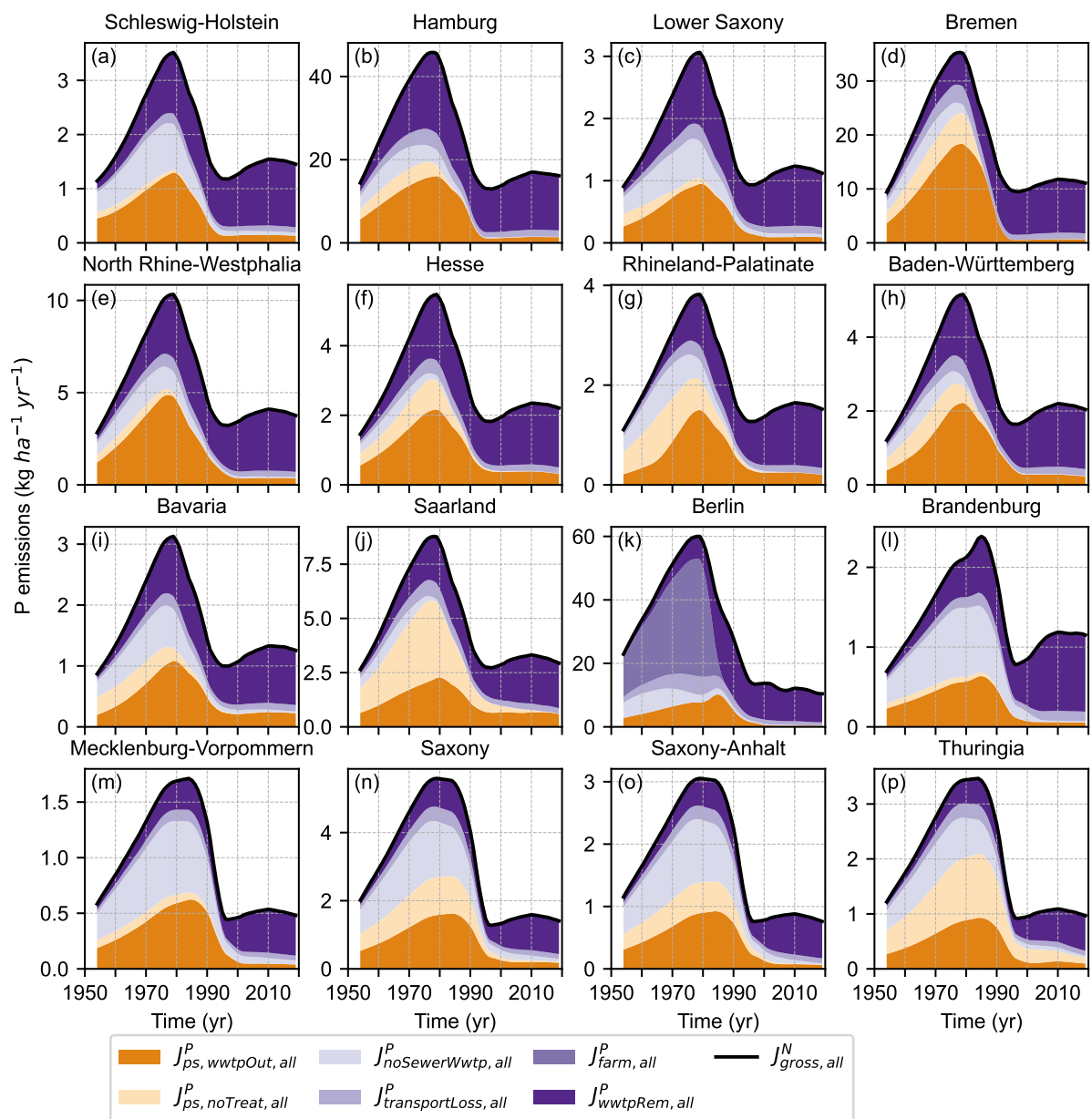
Figure S43. Fate of the P gross emissions at NUTS-1 level for the period 1954–2019 from the mean of our posterior realisations. All fluxes are shown as 5-year backward moving averages (the value in 1954 corresponds to the average of the values for 1950–1954). The pathways of gross emissions are point sources (red colours) or other pathways (purple colours). The data shown include both domestic and industrial emissions, and both urban and rural emissions. See the definition of the notations in the caption of Fig. S41. © Authors 2024. This figure is distributed under a CC BY-NC-SA 4.0 License.
