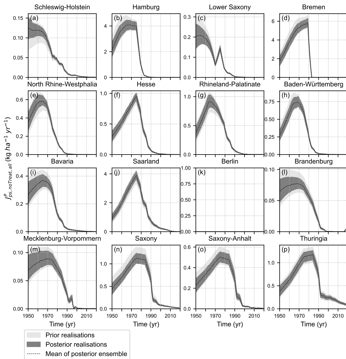
Figure S52. P point source emissions that are collected in the public sewer system but that are not treated in WWTPs J_{ps, NoTreat, all}^P , including both the urban and rural components, and the domestic and industrial/commercial components, from the prior and posterior model realisations at NUTS-1 level for the period 1950–2019. The shaded areas delineate the minimum and maximum values of the 100,000 prior realisations (light grey) and the 100 posterior realisations (dark grey). © Authors 2024. This figure is distributed under a CC BY-NC-SA 4.0 License.
