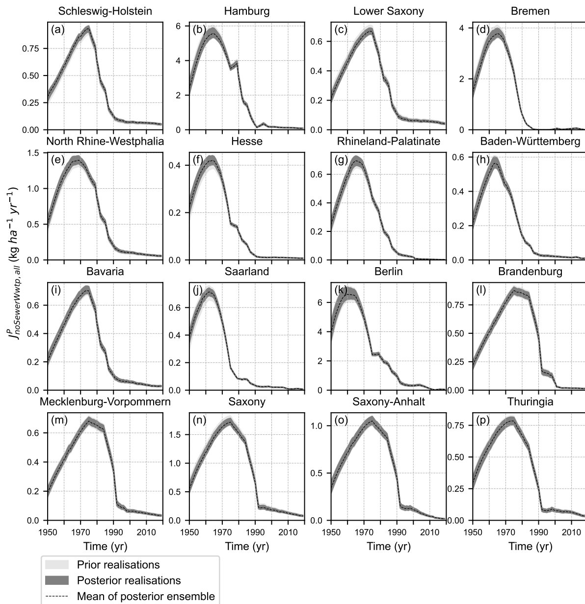
Figure S56. P gross emissions that are not collected in the sewer system nor treated in WWTPs J_{noSewerWwtp,all}^P , including both the urban and rural components, and the domestic and industrial/commercial components, from the prior and posterior model realisations at NUTS-1 level for the period 1950–2019. The shaded areas delineate the minimum and maximum values of the 100,000 prior realisations (light grey) and the 100 posterior realisations (dark grey). © Authors 2024. This figure is distributed under a CC BY-NC-SA 4.0 License.
