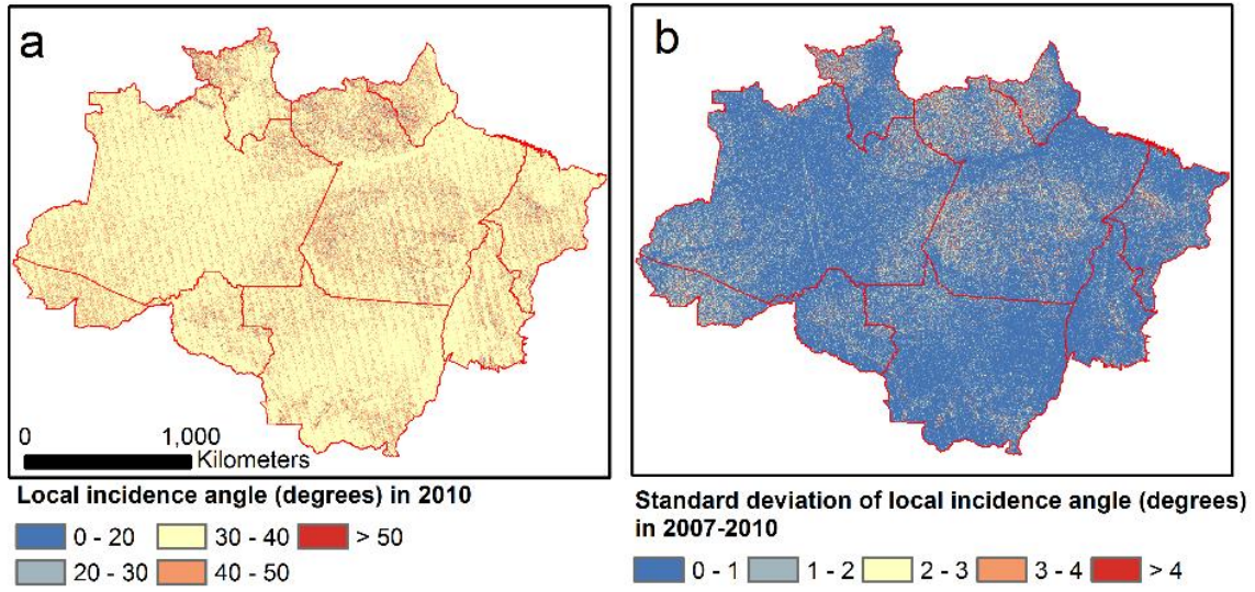
Fig. S1. Spatial distribution maps of ALOS PALSAR data local incidence angle in 2010 (a) and the standard deviation of local incidence angle from 2007 to 2010 (b).
