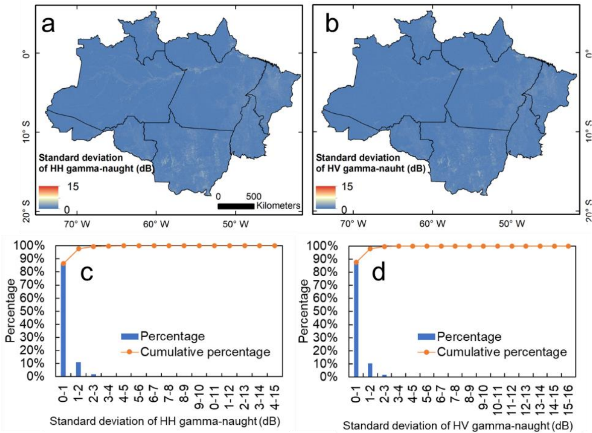
Fig. S2. Spatial distribution maps of the standard deviation of PALSAR HH and HV gamma-naught (a, b) and their histograms (c, d) during 2007-2010.
