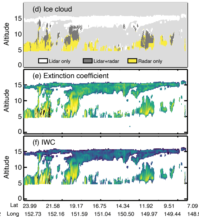
2C-ICE (R05)
