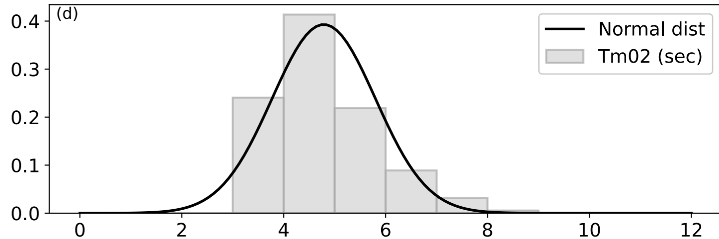
Tm02 [median = 4.6 sec, max = 9.8 sec]
