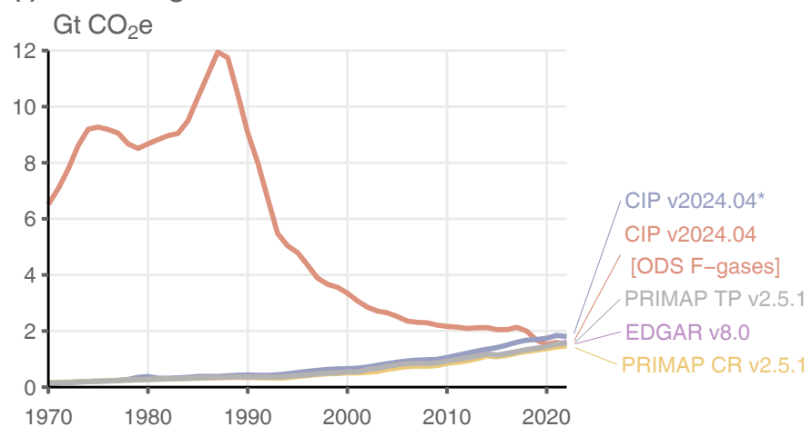
(f) Global F-gas emissions
