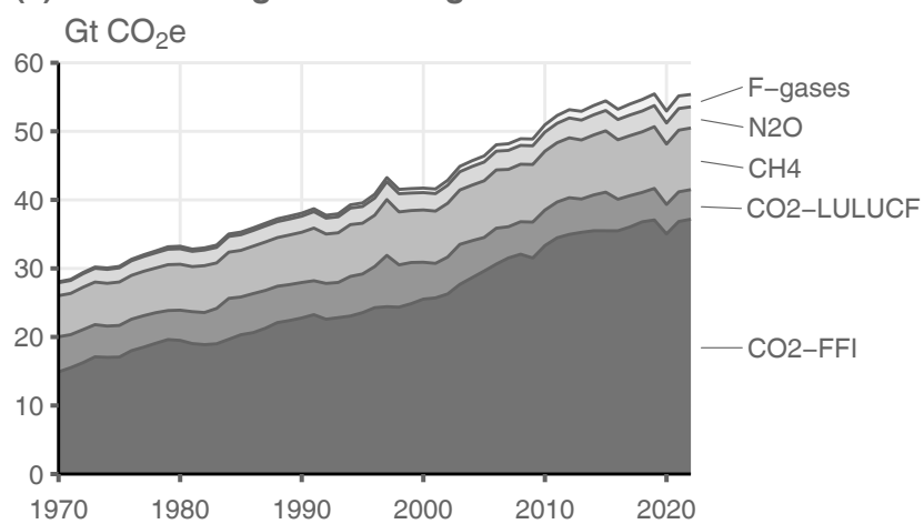
(a) Global total greenhouse gas emissions
