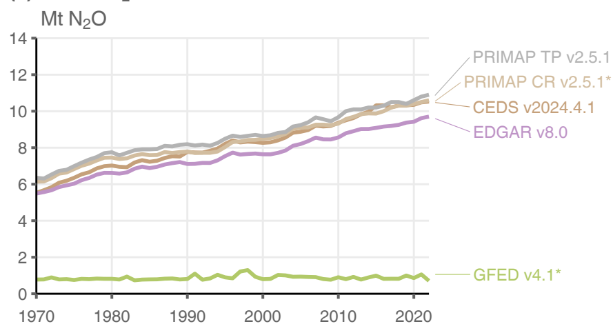
(e) Global N 2 O emissions
