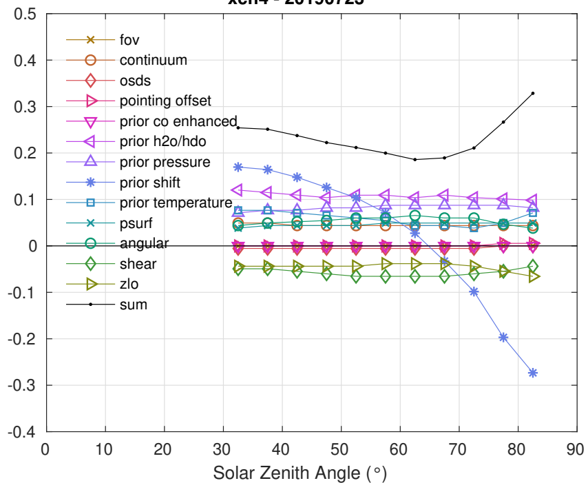
xch4 - 20190723
