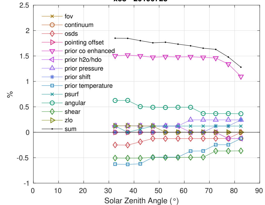
xco - 20190723
