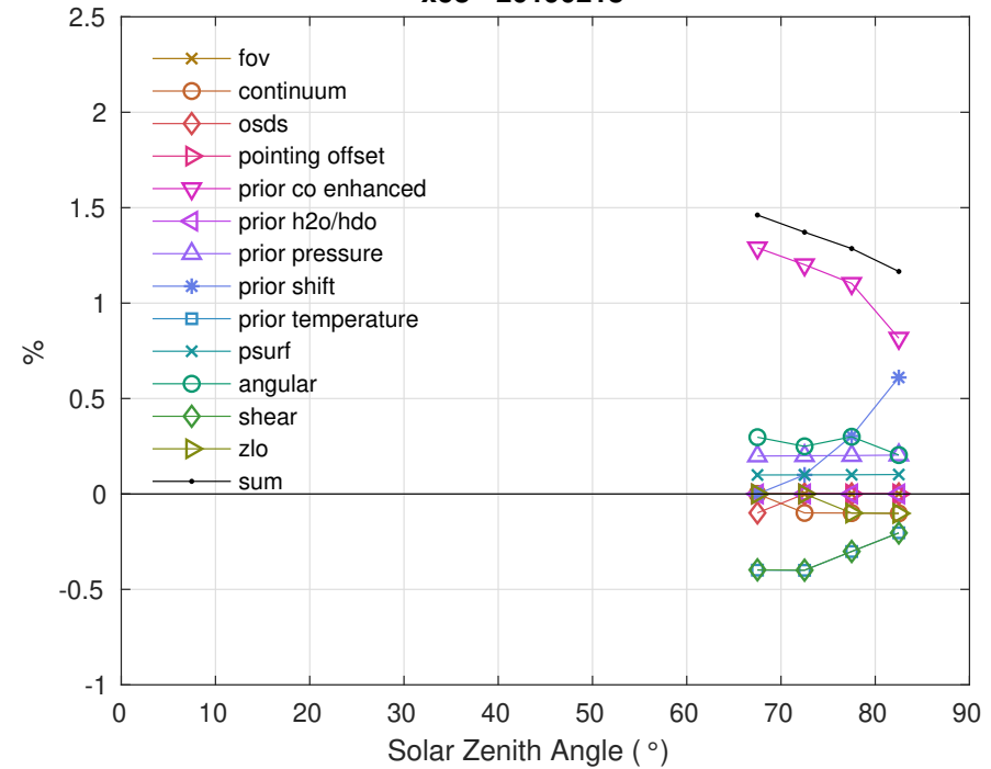
xco - 20190218
