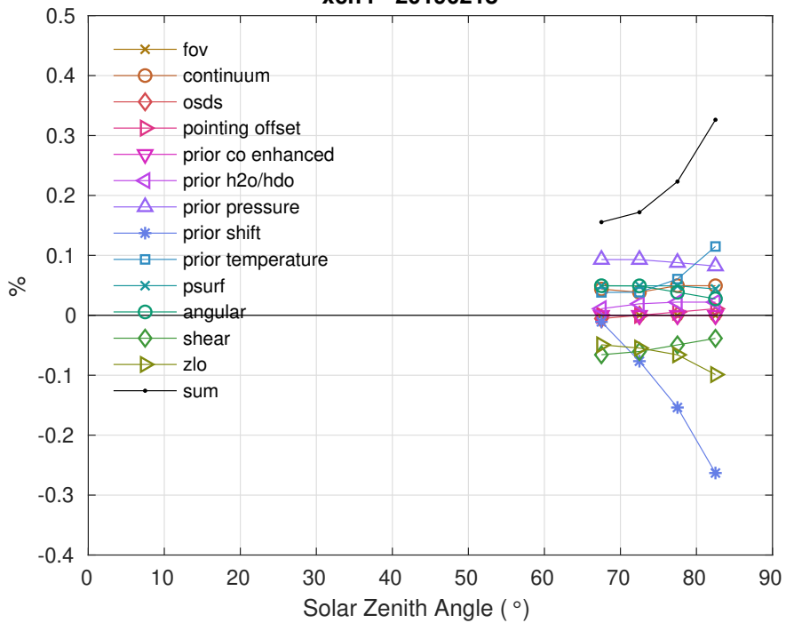
xch4 - 20190218
