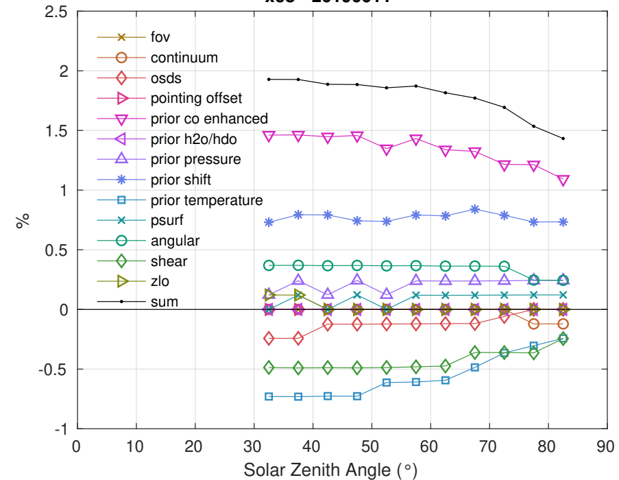
xco - 20190611
