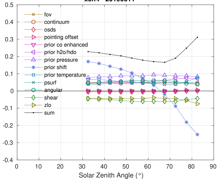
xch4 - 20190611
