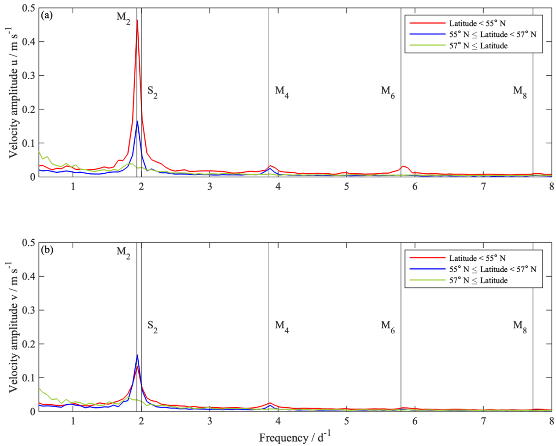
Figure S1: Spectral analysis using a Fourier transform of (a) zonal u and (b) meridional v drifter velocities averaged over trajectories. The periods of the semidiurnal and shallow water tidal components are indicated by the vertical lines.
