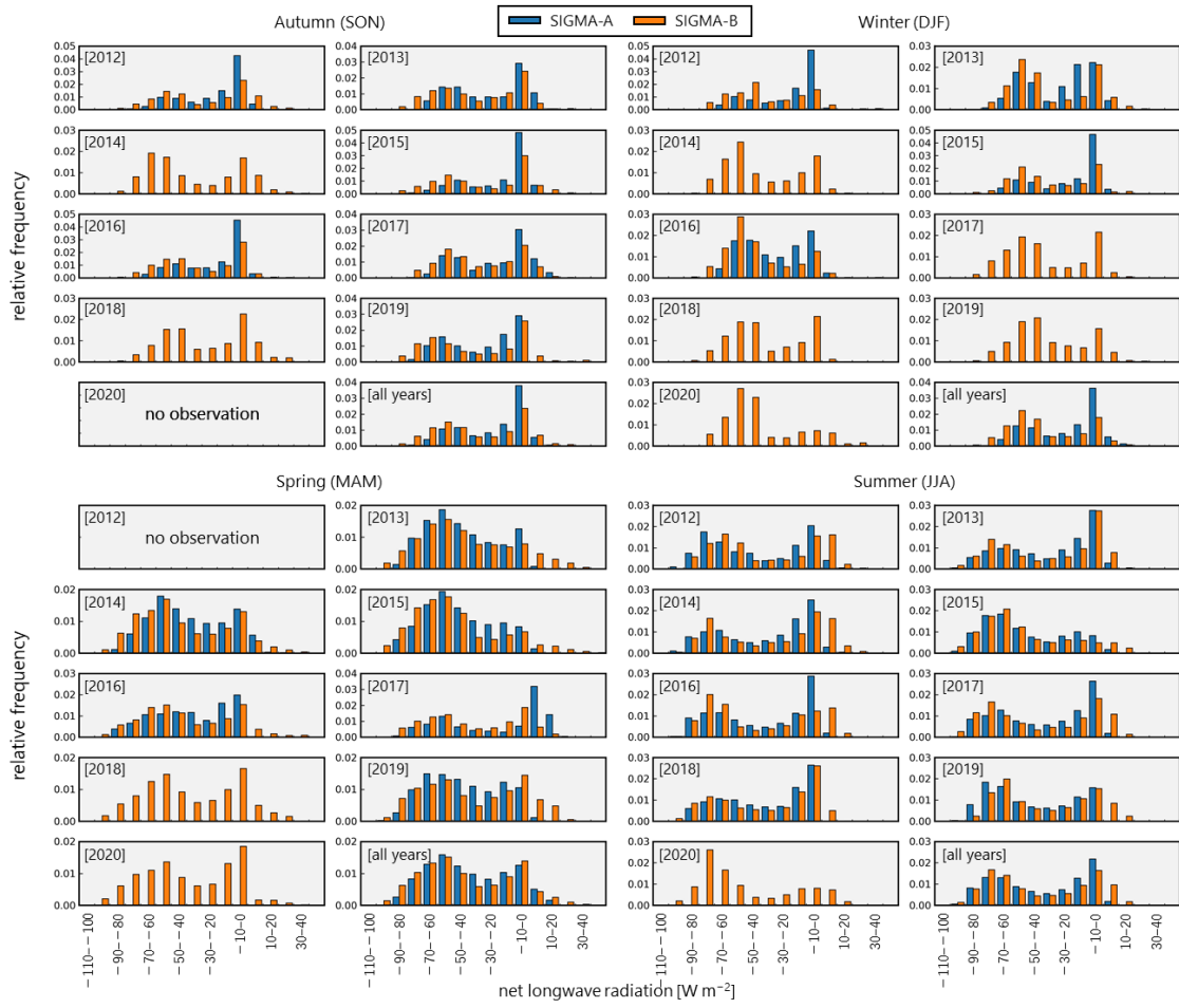
6 7 Figure S2. Histograms of net longwave radiation ( LW_{net} ) in each season and year at the SIGMA-A 8 (blue) and SIGMA-B (orange) sites.
