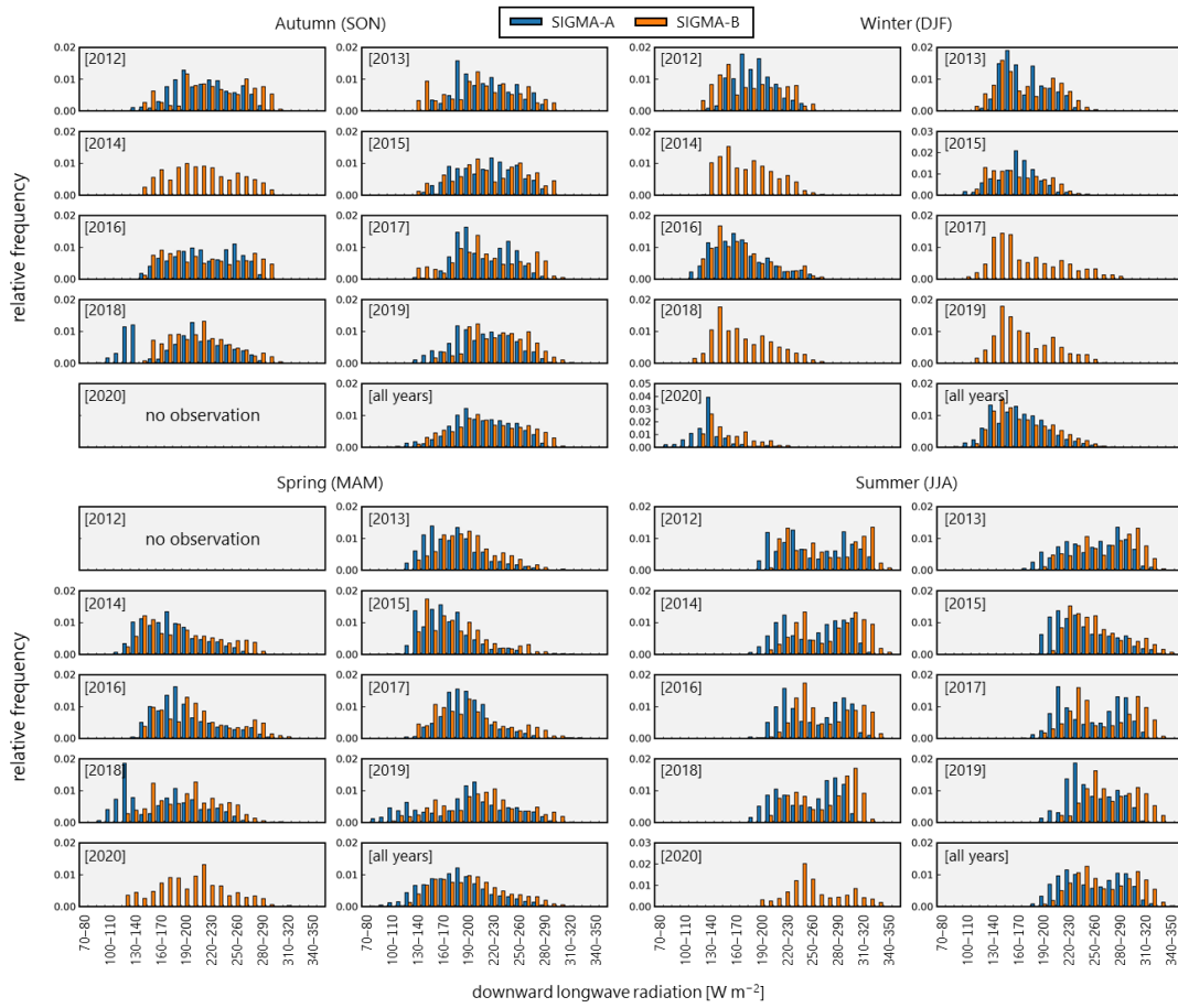
3 Figure S1. Histograms of downward longwave radiation ( LW_d ) in each season and year at the SIGMA- 4 A (blue) and SIGMA-B (orange) sites. If more than half of the observation data were masked, the data 5 were not plotted.
