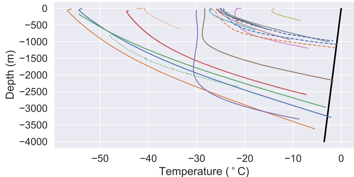
Ice core borehole temperature data
