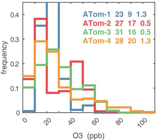
CPacific 0-6 km
