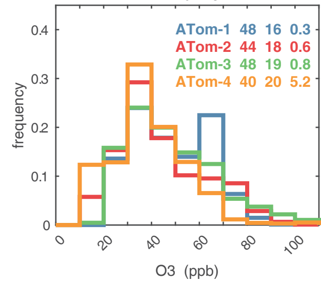
TAtlantic
