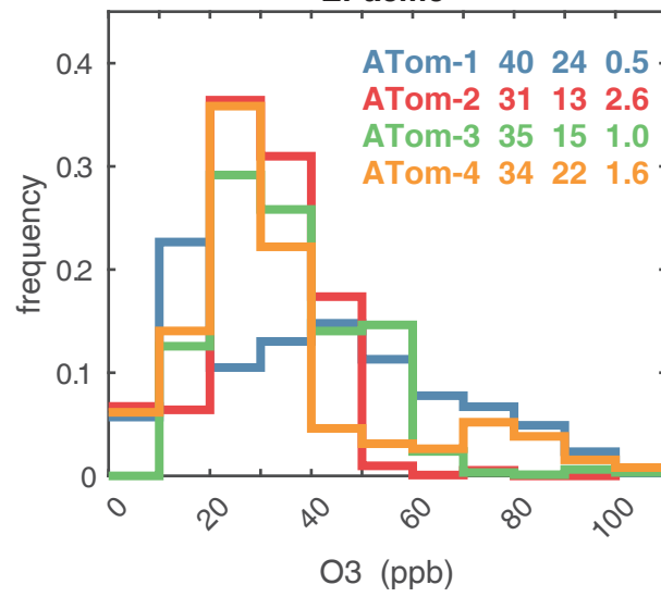
EPacific
