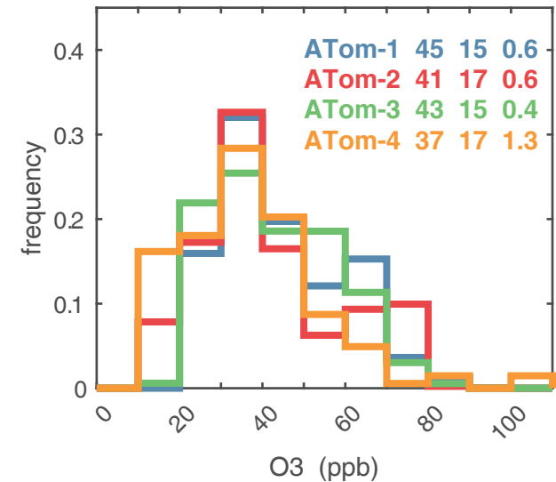
TAtlantic 0-6 km
