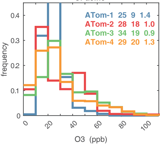
CPacific
