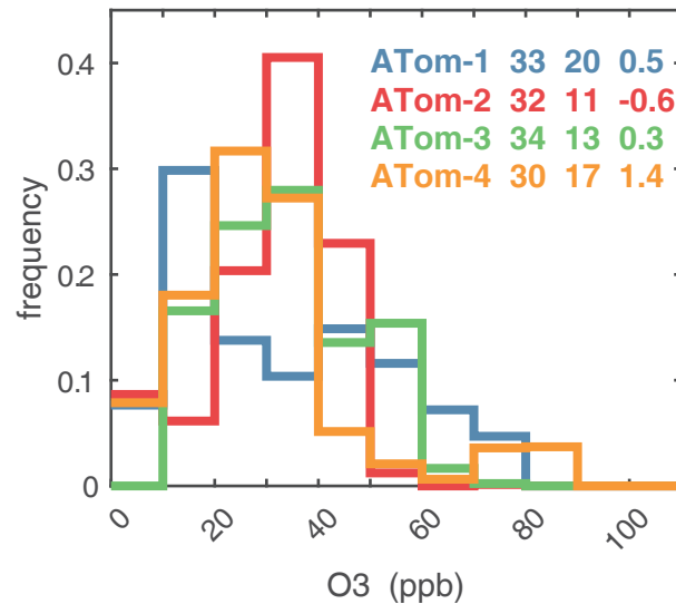
EPacific 0-6 km
