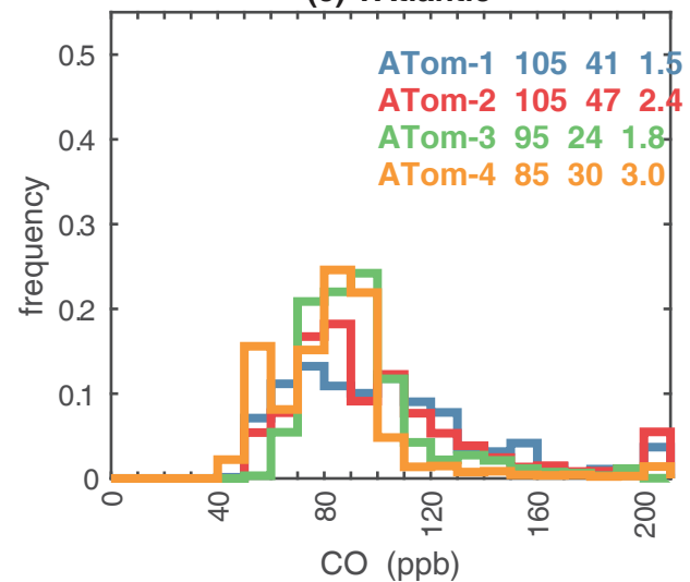
(c) TAtlantic
