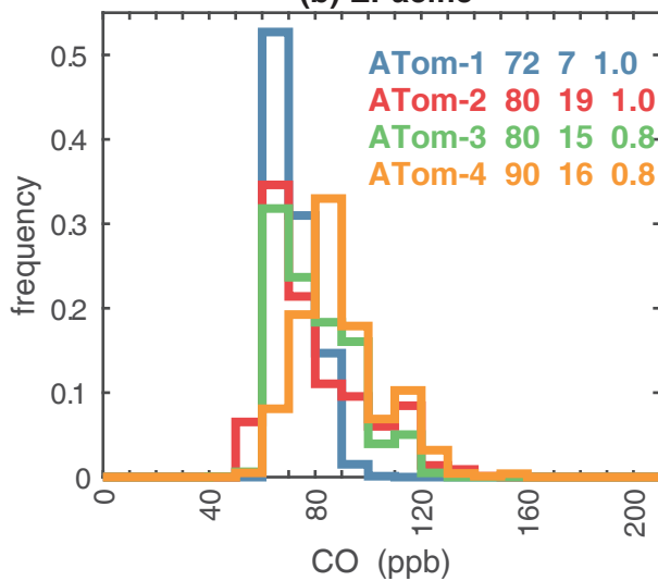
(b) EPacific
