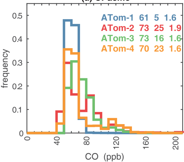
(a) CPacific
